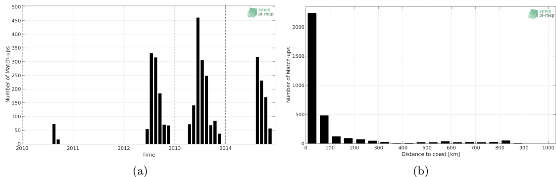
Figure 1: Number of match-ups between Marine mammals and SMOS SSS L3 v5 - 9 Days (CATDS-CECOS-LOCEAN) SSS as a function of time (a) and as function of the distance to coast (b) over the South Pacific Ocean Pi-MEP region and for the full satellite product period.
