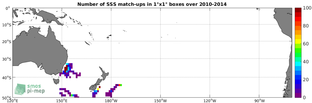
Figure 4: Number of SSS match-ups between Marine mammals SSS and the SMOS SSS L3 v5 - 9 Days (CATDS-CECOS-LOCEAN) SSS product for the South Pacific Ocean Pi-MEP region over 1^\circ \times 1^\circ boxes and for the full satellite product period.
