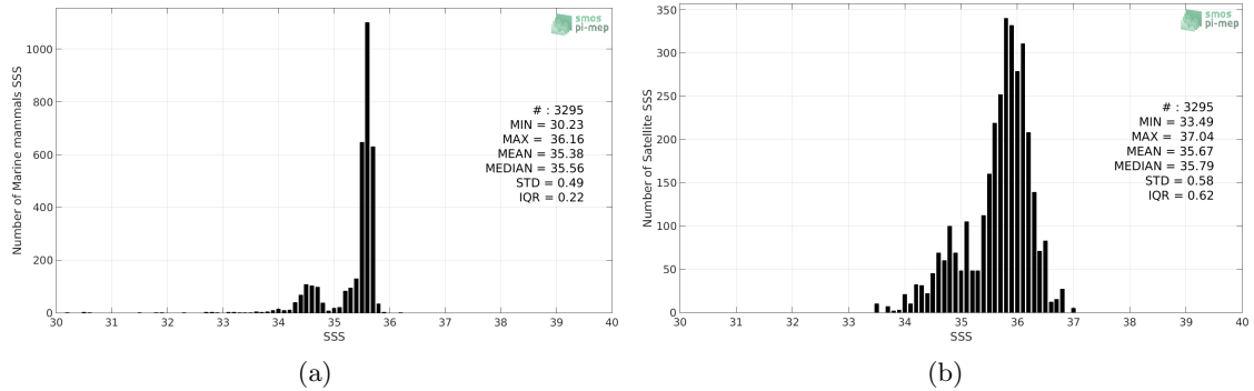
Figure 2: Histograms of SSS from Marine mammals (a) and SMOS SSS L3 v5 - 9 Days (CATDS-CECOS-LOCEAN) (b) considering all match-up pairs per bins of 0.1 over the South Pacific Ocean Pi-MEP region and for the full satellite product period.
