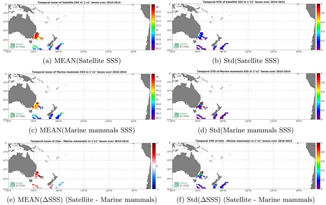
Figure 6: Temporal mean (left) and Std (right) of SSS from SMOS SSS L3 v5 - 9 Days (CATDS-CECOS-LOCEAN) (top), Marine mammals (middle), and of \Delta SSS (Satellite - Marine mammals). Only match-up pairs are used to generate these maps.
