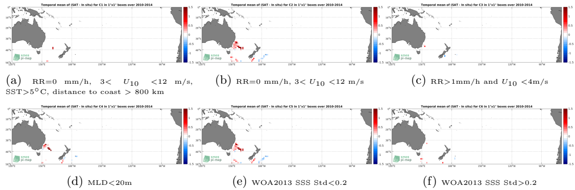
Figure 12: Temporal mean gridded over spatial boxes of size 1^{\circ}\times 1^{\circ} of \Delta\text{SSS} (SMOS SSS L3 v5 - 9 Days (CATDS-CECOS-LOCEAN) - Marine mammals) for 6 different subdatasets corresponding to:RR=0 mm/h, 3 < U_{10} < 12 m/s, SST >5^{\circ}\text{C} , distance to coast > 800 km (a), RR=0 mm/h, 3 < U_{10} < 12 m/s (b), RR >1 mm/h and U_{10} < 4 m/s (c),MLD <20 m (d),WOA2013 SSS Std <0.2 (e),WOA2013 SSS Std >0.2 (f).
