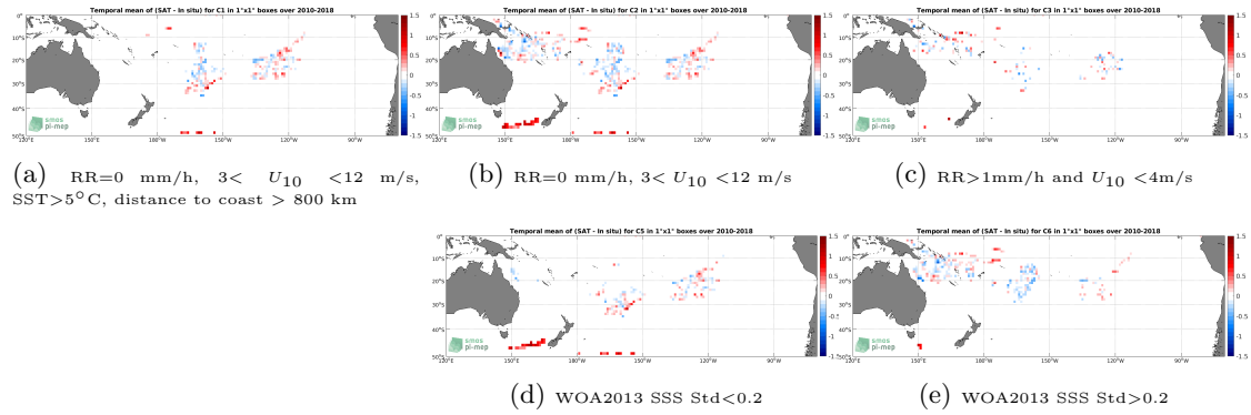
Figure 11: Temporal mean gridded over spatial boxes of size 1^\circ \times 1^\circ of \Delta SSS (SMOS SSS L3 v5 - 9 Days (CATDS-CECOS-LOCEAN) - Surface drifters) for 5 different subdatasets corresponding to:RR=0 mm/h, 3 < U_{10} < 12 m/s, SST >5^\circ\text{C} , distance to coast > 800 km (a), RR=0 mm/h, 3 < U_{10} < 12 m/s (b), RR >1 mm/h and U_{10} < 4 m/s (c), WOA2013 SSS Std <0.2 (d), WOA2013 SSS Std >0.2 (e).
