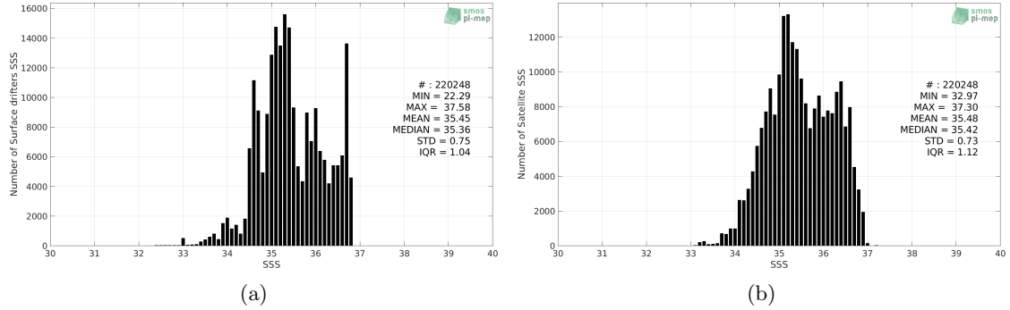
Figure 2: Histograms of SSS from Surface drifters (a) and SMOS SSS L3 v5 - 9 Days (CATDS-CECOS-LOCEAN) (b) considering all match-up pairs per bins of 0.1 over the South Pacific Ocean Pi-MEP region and for the full satellite product period.
