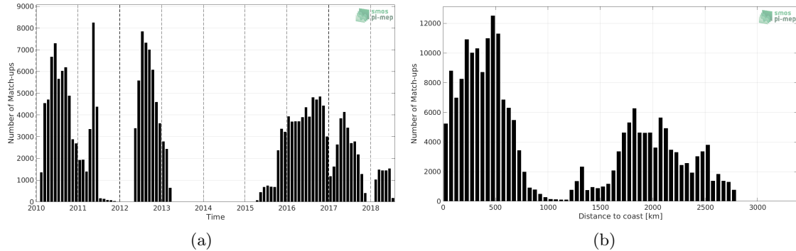
Figure 1: Number of match-ups between Surface drifters and SMOS SSS L3 v5 - 9 Days (CATDS-CECOS-LOCEAN) SSS as a function of time (a) and as function of the distance to coast (b) over the South Pacific Ocean Pi-MEP region and for the full satellite product period.
