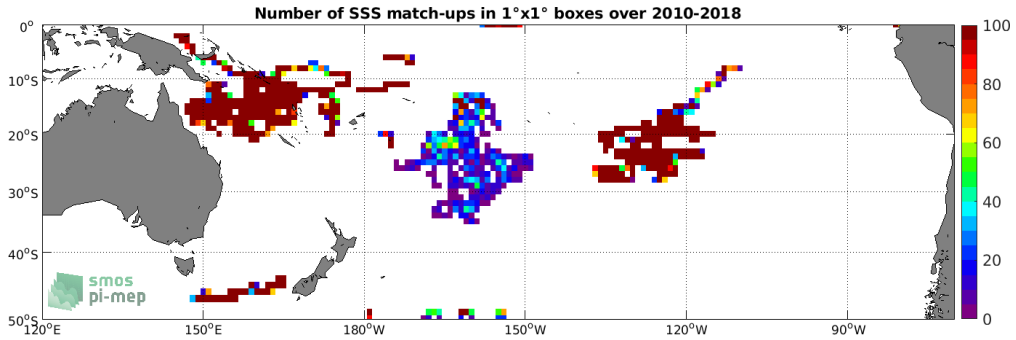
Figure 3: Number of SSS match-ups between Surface drifters SSS and the SMOS SSS L3 v5 - 9 Days (CATDS-CECOS-LOCEAN) SSS product for the South Pacific Ocean Pi-MEP region over 1^\circ \times 1^\circ boxes and for the full satellite product period.
