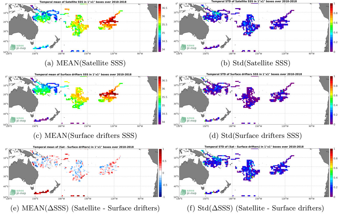
Figure 5: Temporal mean (left) and Std (right) of SSS from SMOS SSS L3 v5 - 9 Days (CATDS-CECOS-LOCEAN) (top), Surface drifters (middle), and of \Delta SSS (Satellite - Surface drifters). Only match-up pairs are used to generate these maps.
