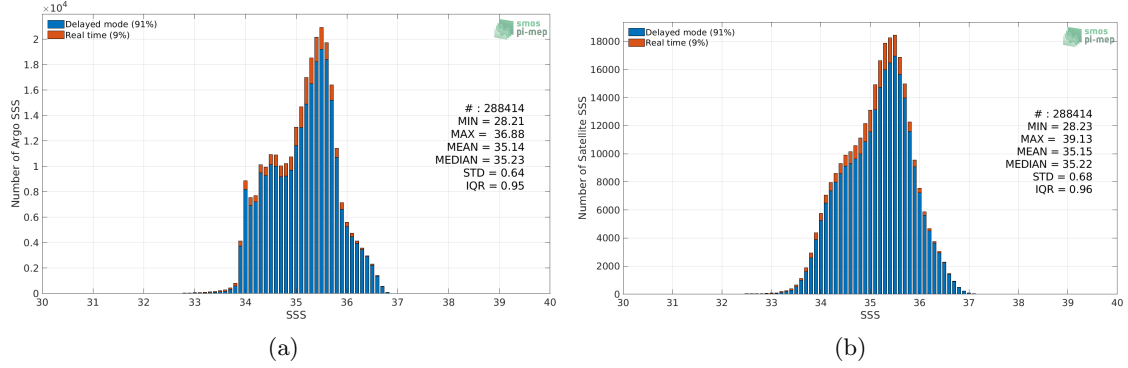
Figure 2: Histograms of SSS from Argo (a) and SMOS SSS L3 v5 - 9 Days (CATDS-CECOS-LOCEAN) (b) considering all match-up pairs per bins of 0.1 over the South Pacific Ocean Pi-MEP region and for the full satellite product period.
