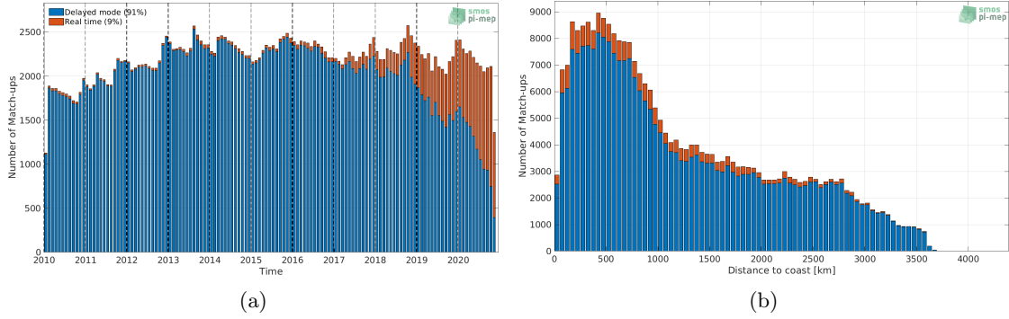
Figure 1: Number of match-ups between Argo and SMOS SSS L3 v5 - 9 Days (CATDS-CECOS-LOCEAN) SSS as a function of time (a) and as function of the distance to coast (b) over the South Pacific Ocean Pi-MEP region and for the full satellite product period.
