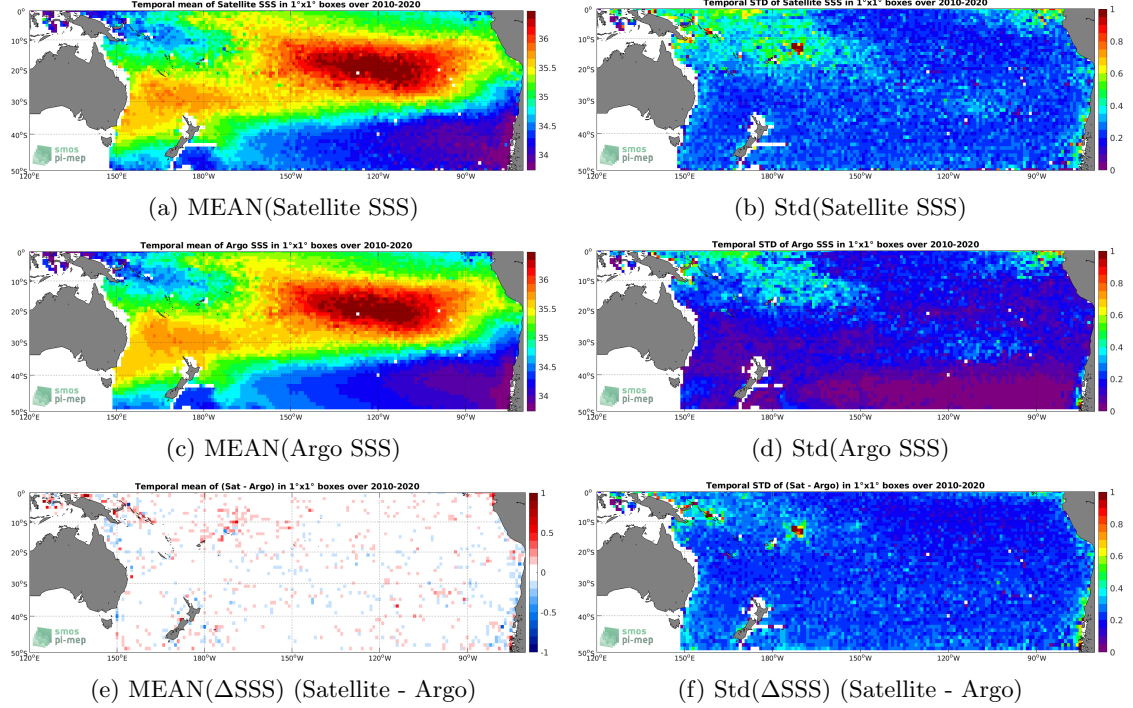
Figure 6: Temporal mean (left) and Std (right) of SSS from SMOS SSS L3 v5 - 9 Days (CATDS-CECOS-LOCEAN) (top), Argo (middle), and of \Delta SSS (Satellite - Argo). Only match-up pairs are used to generate these maps.
