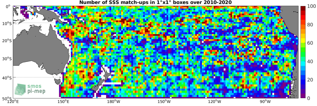
Figure 4: Number of SSS match-ups between Argo SSS and the SMOS SSS L3 v5 - 9 Days (CATDS-CECOS-LOCEAN) SSS product for the South Pacific Ocean Pi-MEP region over 1^\circ \times 1^\circ boxes and for the full satellite product period.
