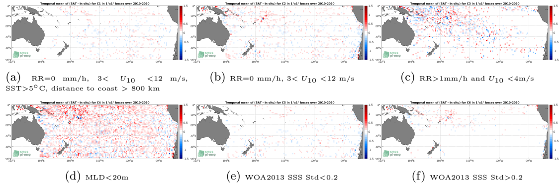
Figure 12: Temporal mean gridded over spatial boxes of size 1^\circ \times 1^\circ of \Delta SSS (SMOS SSS L3 v5 - 9 Days (CATDS-CECOS-LOCEAN) - Argo) for 6 different subdatasets corresponding to: RR=0 mm/h, 3 < U_{10} < 12 m/s, SST > 5^\circ C , distance to coast > 800 km (a), RR=0 mm/h, 3 < U_{10} < 12 m/s (b), RR > 1 mm/h and U_{10} < 4 m/s (c), MLD < 20 m (d), WOA2013 SSS Std < 0.2 (e), WOA2013 SSS Std > 0.2 (f).
