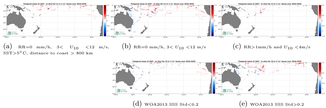
Figure 12: Temporal mean gridded over spatial boxes of size 1^\circ \times 1^\circ of \Delta\text{SSS} (SMOS SSS L3 v5 - 18 Days (CATDS-CECOS-LOCEAN) - TSG (SAMOS)) for 5 different subdatasets corresponding to:RR=0 mm/h, 3 < U_{10} < 12 m/s, SST >5^\circ\text{C} , distance to coast > 800 km (a), RR=0 mm/h, 3 < U_{10} < 12 m/s (b), RR >1 mm/h and U_{10} < 4 m/s (c), WOA2013 SSS Std <0.2 (d), WOA2013 SSS Std >0.2 (e).
