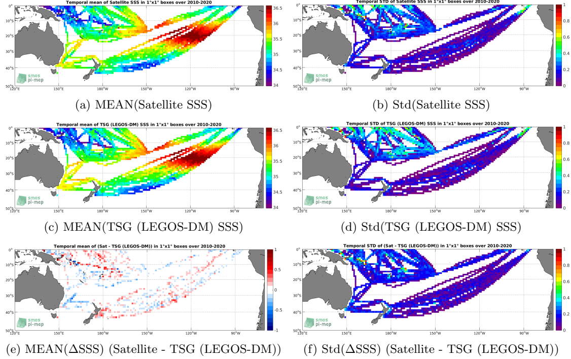
Figure 6: Temporal mean (left) and Std (right) of SSS from SMOS SSS L3 v5 - 18 Days (CATDS-CECOS-LOCEAN) (top), TSG (LEGOS-DM) (middle), and of \Delta\text{SSS} (Satellite - TSG (LEGOS-DM)). Only match-up pairs are used to generate these maps.
