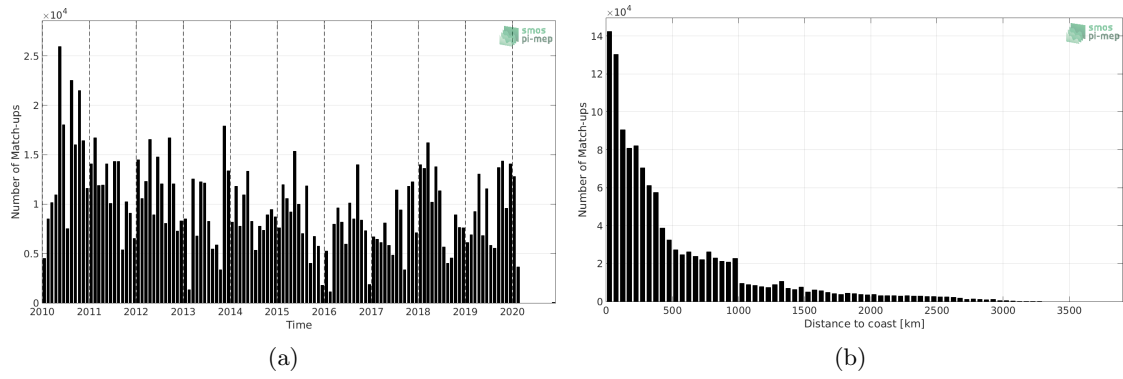
Figure 1: Number of match-ups between TSG (LEGOS-DM) and SMOS SSS L3 v5 - 18 Days (CATDS-CECOS-LOCEAN) SSS as a function of time (a) and as function of the distance to coast (b) over the South Pacific Ocean Pi-MEP region and for the full satellite product period.
