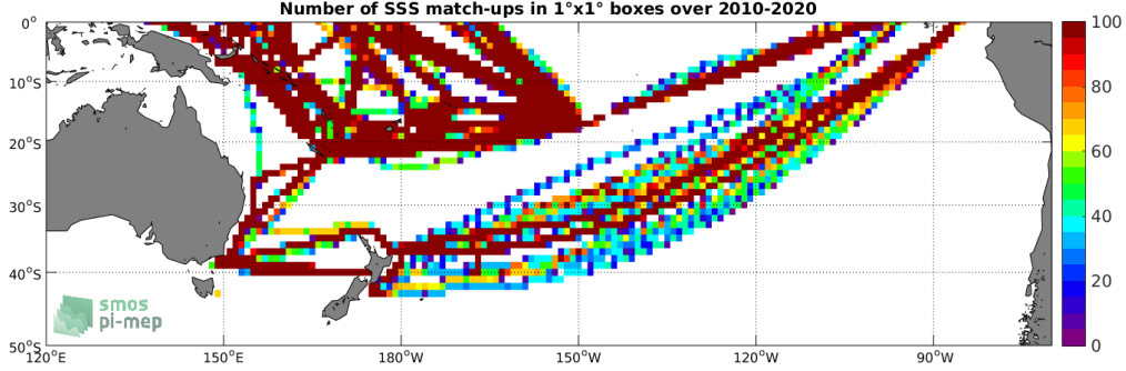
Figure 4: Number of SSS match-ups between TSG (LEGOS-DM) SSS and the SMOS SSS L3 v5 - 18 Days (CATDS-CECOS-LOCEAN) SSS product for the South Pacific Ocean Pi-MEP region over 1^\circ \times 1^\circ boxes and for the full satellite product period.
