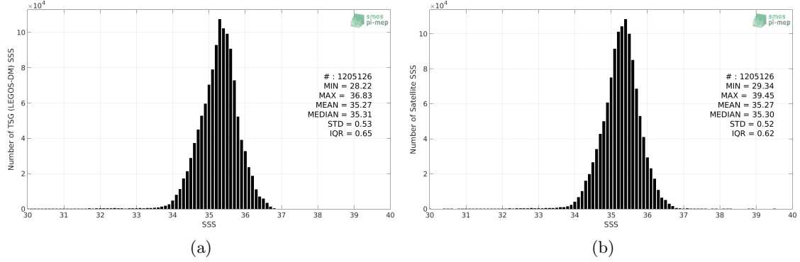
Figure 2: Histograms of SSS from TSG (LEGOS-DM) (a) and SMOS SSS L3 v5 - 18 Days (CATDS-CECOS-LOCEAN) (b) considering all match-up pairs per bins of 0.1 over the South Pacific Ocean Pi-MEP region and for the full satellite product period.
