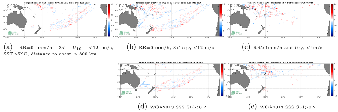
Figure 12: Temporal mean gridded over spatial boxes of size 1^\circ \times 1^\circ of \Delta SSS (SMOS SSS L3 v5 - 18 Days (CATDS-CECOS-LOCEAN) - TSG (LEGOS-DM)) for 5 different subdatasets corresponding to: RR=0 mm/h, 3 < U_{10} < 12 m/s, SST >5^\circ\text{C} , distance to coast > 800 km (a), RR=0 mm/h, 3 < U_{10} < 12 m/s (b), RR>1\text{mm/h} and U_{10} < 4\text{m/s} (c), WOA2013 SSS Std <0.2 (d), WOA2013 SSS Std >0.2 (e).
