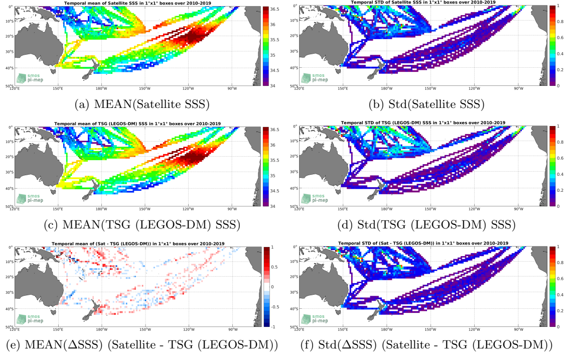
Figure 6: Temporal mean (left) and Std (right) of SSS from SMOS SSS L3 v5 - 18 Days (CATDS-CECOS-LOCEAN) (top), TSG (LEGOS-DM) (middle), and of \Delta SSS (Satellite - TSG (LEGOS-DM)). Only match-up pairs are used to generate these maps.
