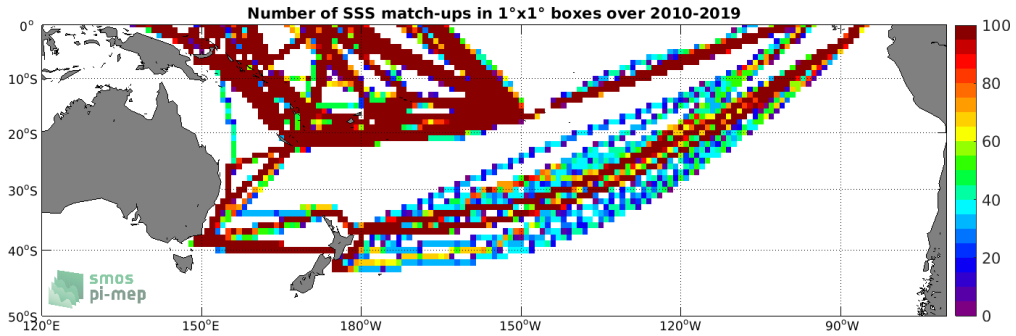
Figure 4: Number of SSS match-ups between TSG (LEGOS-DM) SSS and the SMOS SSS L3 v5 - 18 Days (CATDS-CECOS-LOCEAN) SSS product for the South Pacific Ocean Pi-MEP region over 1°x1° boxes and for the full satellite product period.
