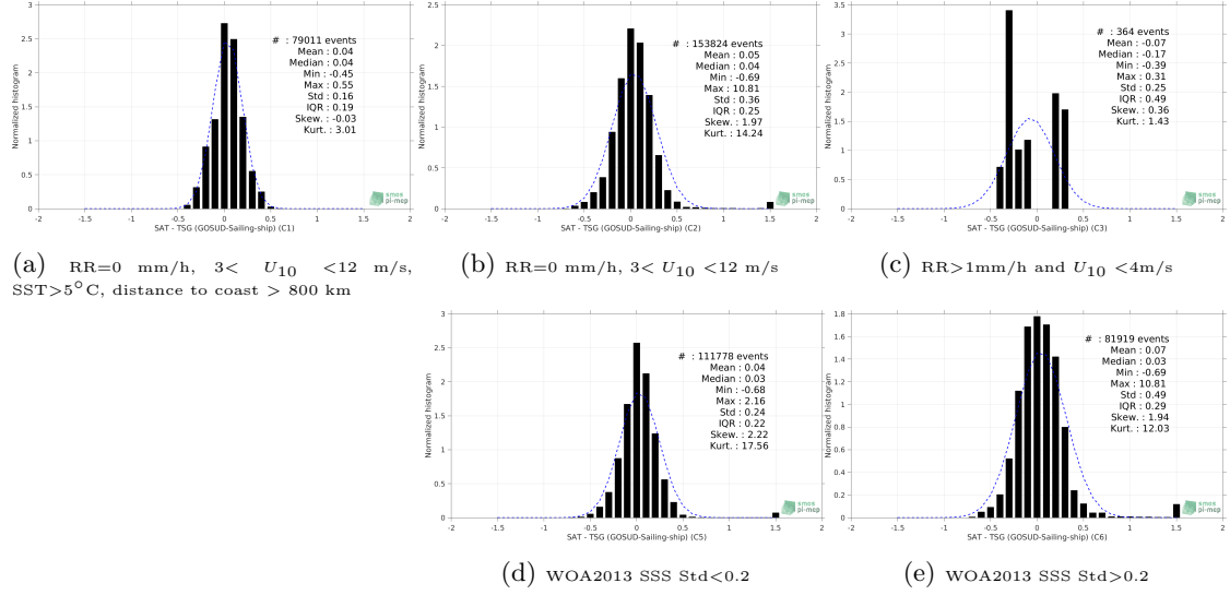
Figure 13: Normalized histogram of \Delta\text{SSS} (SMOS SSS L3 v5 - 18 Days (CATDS-CECOS-LOCEAN) - TSG (GOSUD-Sailing-ship)) for 5 different subdatasets corresponding to: RR=0 mm/h, 3 < U_{10} < 12 m/s, SST > 5^\circ\text{C} , distance to coast > 800 km (a), RR=0 mm/h, 3 < U_{10} < 12 m/s (b), RR > 1\text{mm/h} and U_{10} < 4\text{m/s} (c), WOA2013 SSS Std < 0.2 (d), WOA2013 SSS Std > 0.2 (e).
