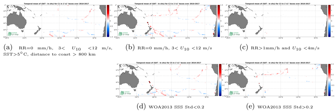
Figure 12: Temporal mean gridded over spatial boxes of size 1^\circ \times 1^\circ of \Delta\text{SSS} (SMOS SSS L3 v5 - 18 Days (CATDS-CECOS-LOCEAN) - TSG (GOSUD-Sailing-ship)) for 5 different subdatasets corresponding to:RR=0 mm/h, 3 < U_{10} < 12 m/s, SST>5°C, distance to coast > 800 km (a), RR=0 mm/h, 3 < U_{10} < 12 m/s (b), RR>1mm/h and U_{10} < 4 m/s (c), WOA2013 SSS Std<0.2 (d), WOA2013 SSS Std>0.2 (e).
