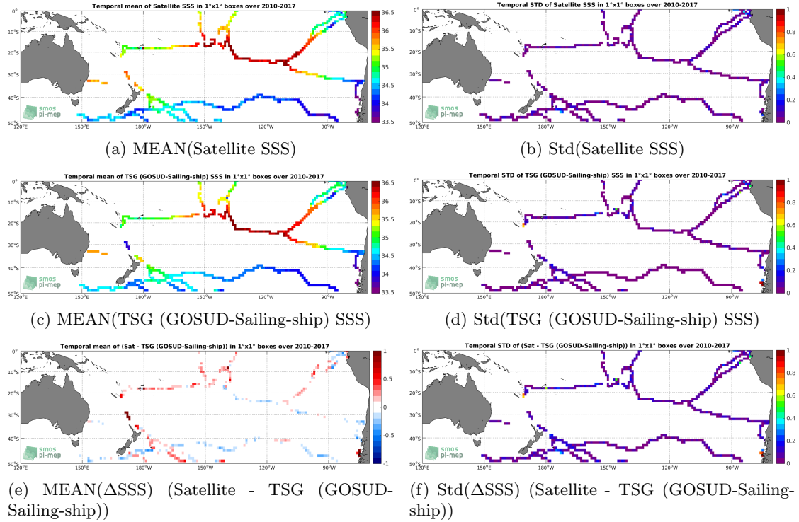
Figure 6: Temporal mean (left) and Std (right) of SSS from SMOS SSS L3 v5 - 18 Days (CATDS-CECOS-LOCEAN) (top), TSG (GOSUD-Sailing-ship) (middle), and of \Delta SSS (Satellite - TSG (GOSUD-Sailing-ship)). Only match-up pairs are used to generate these maps.
