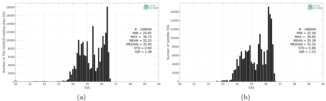
Figure 2: Histograms of SSS from TSG (GOSUD-Sailing-ship) (a) and SMOS SSS L3 v5 - 18 Days (CATDS-CECOS-LOCEAN) (b) considering all match-up pairs per bins of 0.1 over the South Pacific Ocean Pi-MEP region and for the full satellite product period.
