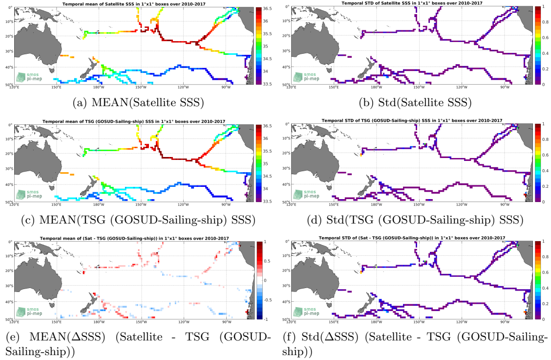
Figure 6: Temporal mean (left) and Std (right) of SSS from SMOS SSS L3 v5 - 18 Days (CATDS-CECOS-LOCEAN) (top), TSG (GOSUD-Sailing-ship) (middle), and of \Delta SSS (Satellite - TSG (GOSUD-Sailing-ship)). Only match-up pairs are used to generate these maps.
