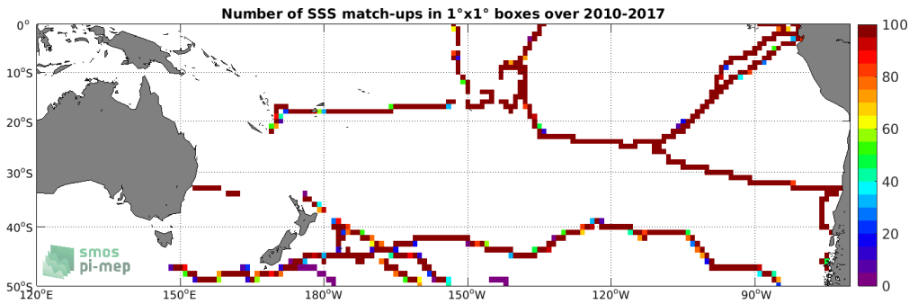
Figure 4: Number of SSS match-ups between TSG (GOSUD-Sailing-ship) SSS and the SMOS SSS L3 v5 - 18 Days (CATDS-CECOS-LOCEAN) SSS product for the South Pacific Ocean Pi-MEP region over 1^\circ \times 1^\circ boxes and for the full satellite product period.
