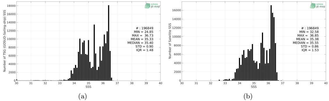
Figure 2: Histograms of SSS from TSG (GOSUD-Sailing-ship) (a) and SMOS SSS L3 v5 - 18 Days (CATDS-CECOS-LOCEAN) (b) considering all match-up pairs per bins of 0.1 over the South Pacific Ocean Pi-MEP region and for the full satellite product period.
