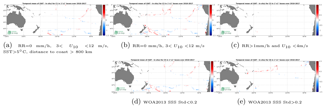
Figure 12: Temporal mean gridded over spatial boxes of size 1^\circ \times 1^\circ of \Delta SSS (SMOS SSS L3 v5 - 18 Days (CATDS-CECOS-LOCEAN) - TSG (GOSUD-Sailing-ship)) for 5 different subdatasets corresponding to: RR=0 mm/h, 3 < U_{10} < 12 m/s, SST > 5°C, distance to coast > 800 km (a), RR=0 mm/h, 3 < U_{10} < 12 m/s (b), RR > 1mm/h and U_{10} < 4 m/s (c), WOA2013 SSS Std < 0.2 (d), WOA2013 SSS Std > 0.2 (e).
