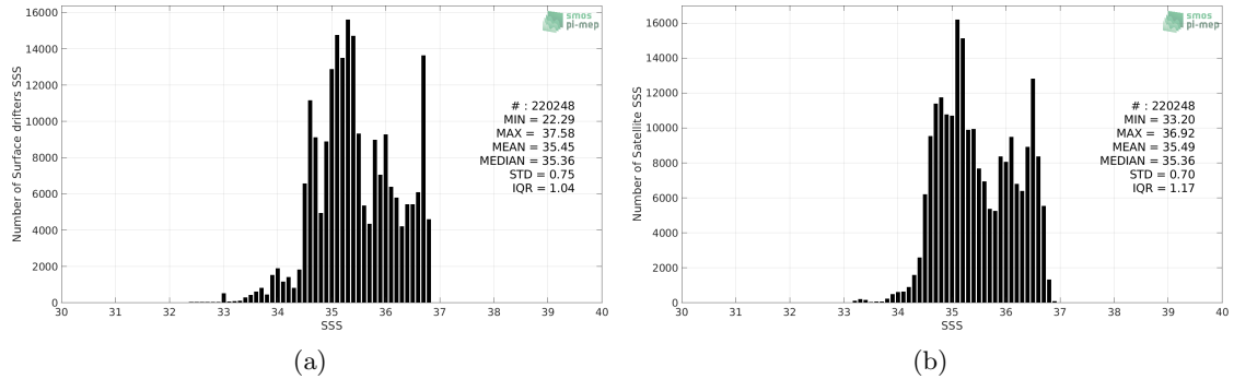
Figure 2: Histograms of SSS from Surface drifters (a) and SMOS SSS L3 v5 - 18 Days (CATDS-CECOS-LOCEAN) (b) considering all match-up pairs per bins of 0.1 over the South Pacific Ocean Pi-MEP region and for the full satellite product period.
