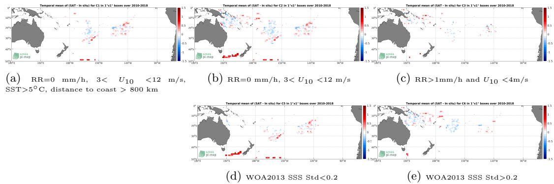
Figure 11: Temporal mean gridded over spatial boxes of size 1^\circ \times 1^\circ of \Delta\text{SSS} (SMOS SSS L3 v5 - 18 Days (CATDS-CECOS-LOCEAN) - Surface drifters) for 5 different subdatasets corresponding to:RR=0 mm/h, 3 < U_{10} < 12 m/s, SST >5^\circ\text{C} , distance to coast > 800 km (a), RR=0 mm/h, 3 < U_{10} < 12 m/s (b), RR >1\text{mm/h} and U_{10} < 4\text{m/s} (c), WOA2013 SSS Std <0.2 (d), WOA2013 SSS Std >0.2 (e).
