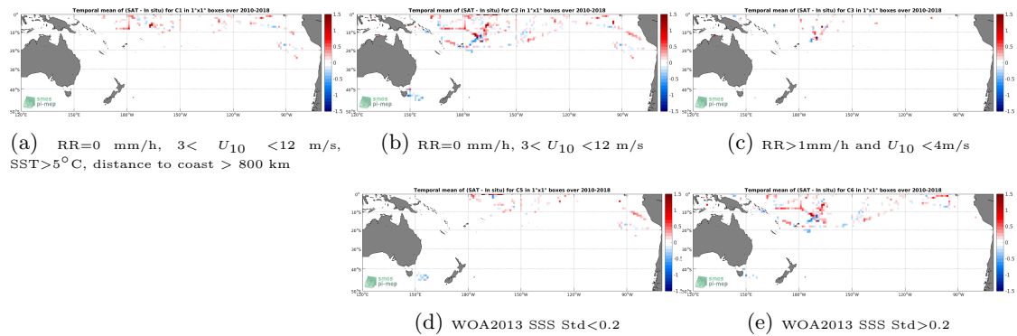
Figure 12: Temporal mean gridded over spatial boxes of size 1^\circ \times 1^\circ of \Delta SSS (SMOS-L3-CATDS-CECOS-LOCEAN-V4-9DAYS-25KM - TSG-SAMOS) for 5 different subdatasets corresponding to:RR=0 mm/h, 3 < U_{10} < 12 m/s, SST >5^\circ C, distance to coast > 800 km (a), RR=0 mm/h, 3 < U_{10} < 12 m/s (b), RR >1 mm/h and U_{10} < 4 m/s (c), WOA2013 SSS Std <0.2 (d), WOA2013 SSS Std >0.2 (e).
