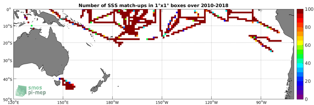
Figure 4: Number of SSS match-ups between TSG-SAMOS SSS and the SMOS-L3-CATDS-CECOS-LOCEAN-V4-9DAYS-25KM SSS product for the South Pacific Ocean Pi-MEP region over 1^\circ \times 1^\circ boxes and for the full satellite product period.
