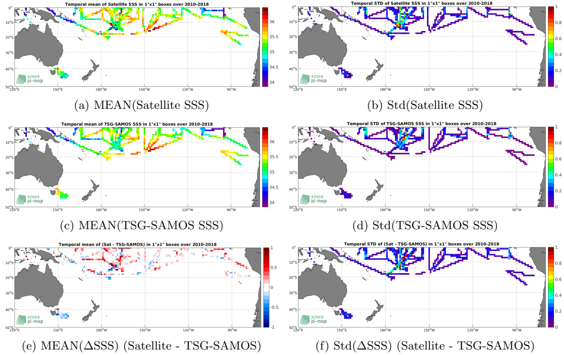
Figure 6: Temporal mean (left) and Std (right) of SSS from SMOS-L3-CATDS-CECOS-LOCEAN-V4-9DAYS-25KM (top), TSG-SAMOS (middle), and of \Delta SSS (Satellite - TSG-SAMOS). Only match-up pairs are used to generate these maps.
