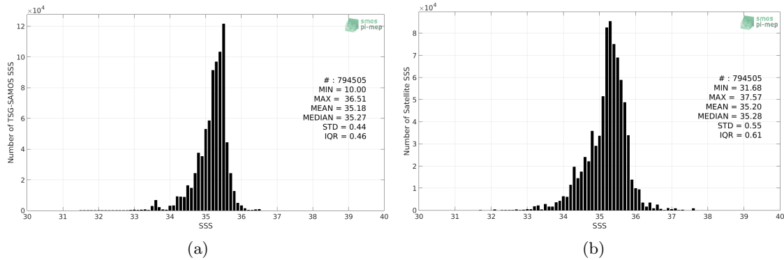
Figure 2: Histograms of SSS from TSG-SAMOS (a) and SMOS-L3-CATDS-CECOS-LOCEAN-V4-9DAYS-25KM (b) considering all match-up pairs per bins of 0.1 over the South Pacific Ocean Pi-MEP region and for the full satellite product period.
