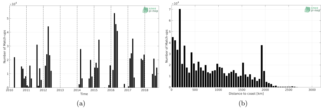
Figure 1: Number of match-ups between TSG-SAMOS and SMOS-L3-CATDS-CECOS-LOCEAN-V4-9DAYS-25KM SSS as a function of time (a) and as function of the distance to coast (b) over the South Pacific Ocean Pi-MEP region and for the full satellite product period.
