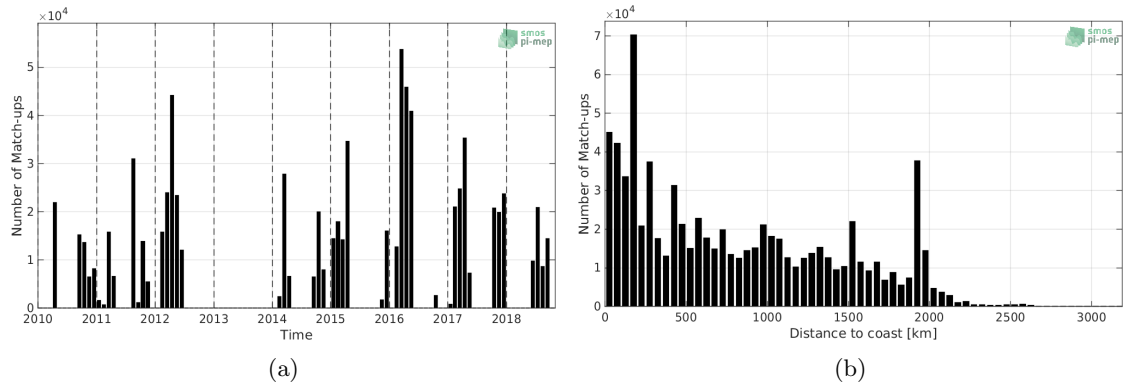
Figure 1: Number of match-ups between TSG-SAMOS and SMOS-L3-CATDS-CECOS-LOCEAN-V4-9DAYS-25KM SSS as a function of time (a) and as function of the distance to coast (b) over the South Pacific Ocean Pi-MEP region and for the full satellite product period.
