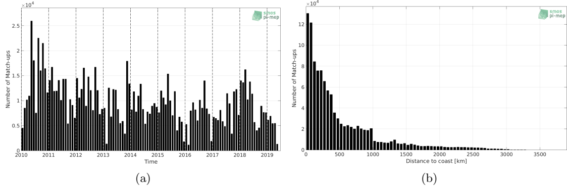
Figure 1: Number of match-ups between TSG (LEGOS-DM) and SMOS SSS L3 v4 - 9 Days (CATDS-CECOS-LOCEAN) SSS as a function of time (a) and as function of the distance to coast (b) over the South Pacific Ocean Pi-MEP region and for the full satellite product period.
