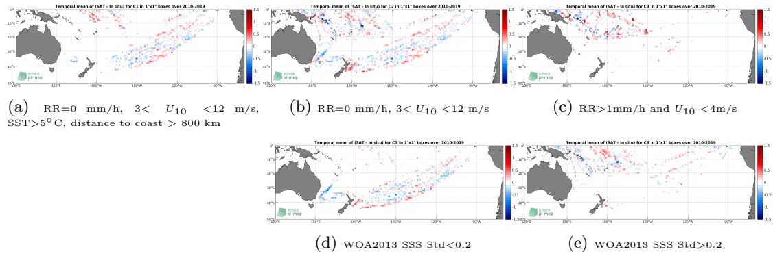
Figure 12: Temporal mean gridded over spatial boxes of size 1^\circ \times 1^\circ of \Delta SSS (SMOS SSS L3 v4 - 9 Days (CATDS-CECOS-LOCEAN) - TSG (LEGOS-DM)) for 5 different subdatasets corresponding to: RR=0 mm/h, 3 < U_{10} < 12 m/s, SST >5^\circ\text{C} , distance to coast > 800 km (a), RR=0 mm/h, 3 < U_{10} < 12 m/s (b), RR>1\text{mm/h} and U_{10} < 4\text{m/s} (c), WOA2013 SSS Std <0.2 (d), WOA2013 SSS Std >0.2 (e).
