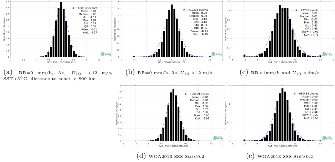
Figure 13: Normalized histogram of \Delta SSS (SMOS SSS L3 v4 - 9 Days (CATDS-CECOS-LOCEAN) - TSG (LEGOS-DM)) for 5 different subdatasets corresponding to: RR=0 mm/h, 3 < U_{10} < 12 m/s, SST>5°C, distance to coast > 800 km (a), RR=0 mm/h, 3 < U_{10} < 12 m/s (b), RR>1mm/h and U_{10} < 4 m/s (c), WOA2013 SSS Std<0.2 (d), WOA2013 SSS Std>0.2 (e).
