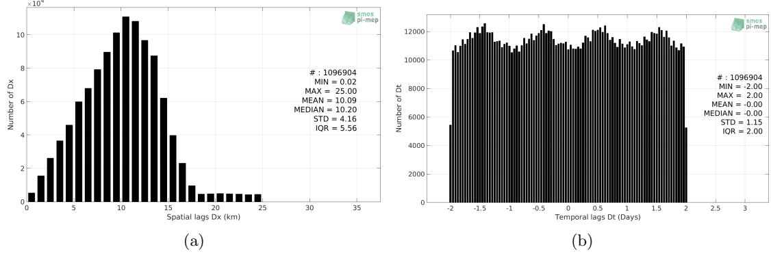
Figure 5: Histograms of the spatial (a) and temporal (b) lags between the time of the TSG (LEGOS-DM) measurements and the date of the corresponding SMOS SSS L3 v4 - 9 Days (CATDS-CECOS-LOCEAN) SSS product.
