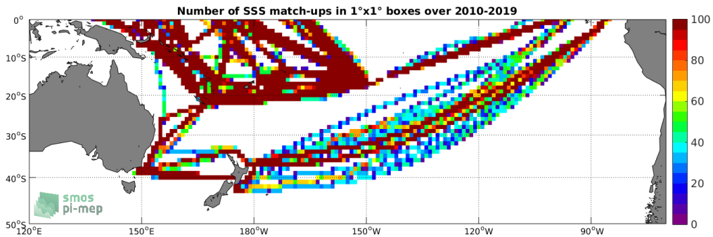
Figure 4: Number of SSS match-ups between TSG (LEGOS-DM) SSS and the SMOS SSS L3 v4 - 9 Days (CATDS-CECOS-LOCEAN) SSS product for the South Pacific Ocean Pi-MEP region over 1°x1° boxes and for the full satellite product period.
