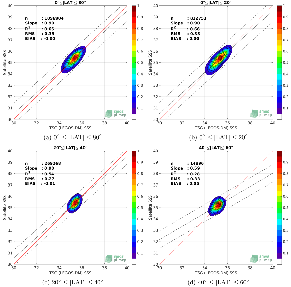
Figure 9: Contour maps of the concentration of SMOS SSS L3 v4 - 9 Days (CATDS-CECOS-LOCEAN) SSS (y-axis) versus TSG (LEGOS-DM) SSS (x-axis) at match-up pairs for different latitude bands. For each plot, the red line shows x=y . The black thin and dashed lines indicate a linear fit through the data cloud and the \pm 95\% confidence levels, respectively. The number match-up pairs n , the slope and R^2 coefficient of the linear fit, the root mean square (RMS) and the mean bias between satellite and in situ data are indicated for each latitude band in each plots.
