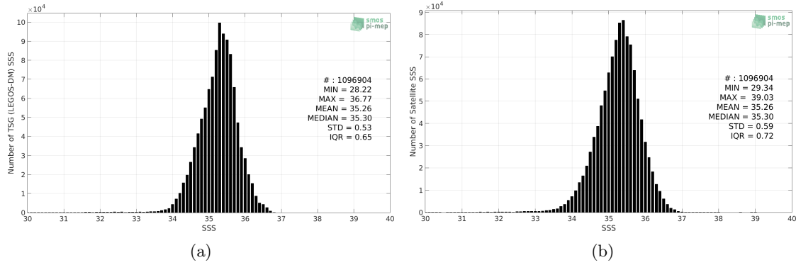
Figure 2: Histograms of SSS from TSG (LEGOS-DM) (a) and SMOS SSS L3 v4 - 9 Days (CATDS-CECOS-LOCEAN) (b) considering all match-up pairs per bins of 0.1 over the South Pacific Ocean Pi-MEP region and for the full satellite product period.
