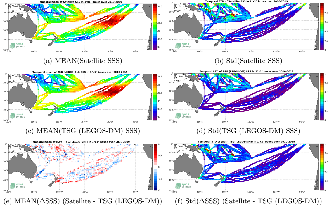
Figure 6: Temporal mean (left) and Std (right) of SSS from SMOS SSS L3 v4 - 9 Days (CATDS-CECOS-LOCEAN) (top), TSG (LEGOS-DM) (middle), and of \Delta SSS (Satellite - TSG (LEGOS-DM)). Only match-up pairs are used to generate these maps.
