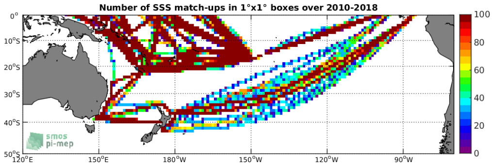
Figure 4: Number of SSS match-ups between TSG-LEGOS-DM SSS and the SMOS-L3-CATDS-CECOS-LOCEAN-V4-9DAYS-25KM SSS product for the South Pacific Ocean Pi-MEP region over 1^\circ \times 1^\circ boxes and for the full satellite product period.
