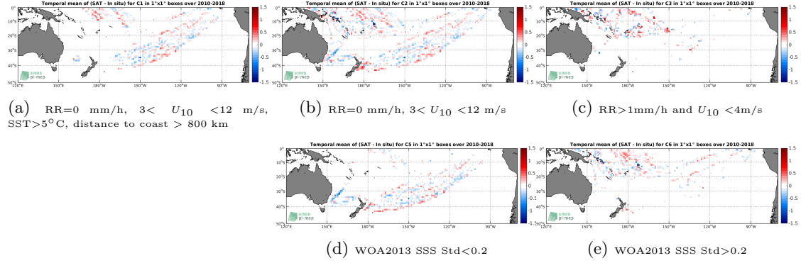
Figure 12: Temporal mean gridded over spatial boxes of size 1^\circ \times 1^\circ of \Delta SSS (SMOS-L3-CATDS-CECOS-LOCEAN-V4-9DAYS-25KM - TSG-LEGOS-DM) for 5 different subdatasets corresponding to: RR=0 mm/h, 3 < U_{10} < 12 m/s, SST > 5^\circ C , distance to coast > 800 km (a), RR=0 mm/h, 3 < U_{10} < 12 m/s (b), RR > 1 mm/h and U_{10} < 4 m/s (c), WOA2013 SSS Std < 0.2 (d), WOA2013 SSS Std > 0.2 (e).
