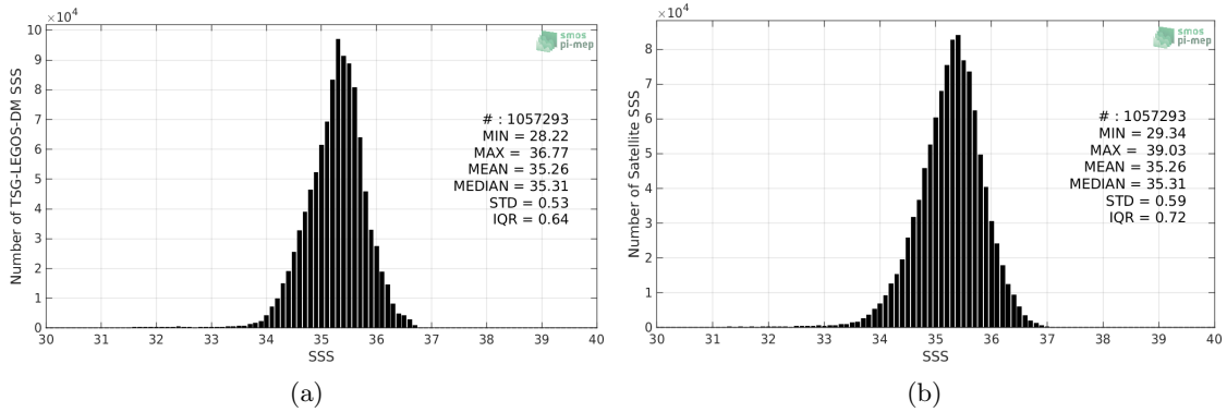
Figure 2: Histograms of SSS from TSG-LEGOS-DM (a) and SMOS-L3-CATDS-CECOS-LOCEAN-V4-9DAYS-25KM (b) considering all match-up pairs per bins of 0.1 over the South Pacific Ocean Pi-MEP region and for the full satellite product period.
