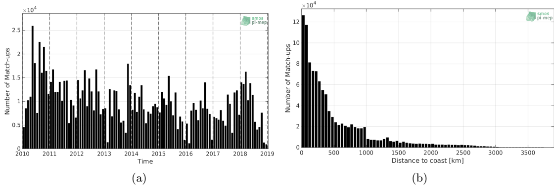
Figure 1: Number of match-ups between TSG-LEGOS-DM and SMOS-L3-CATDS-CECOS-LOCEAN-V4-9DAYS-25KM SSS as a function of time (a) and as function of the distance to coast (b) over the South Pacific Ocean Pi-MEP region and for the full satellite product period.
