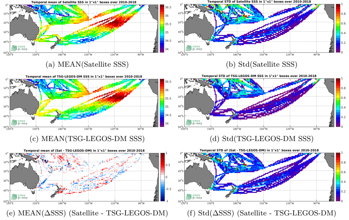
Figure 6: Temporal mean (left) and Std (right) of SSS from SMOS-L3-CATDS-CECOS-LOCEAN-V4-9DAYS-25KM (top), TSG-LEGOS-DM (middle), and of \Delta SSS (Satellite - TSG-LEGOS-DM). Only match-up pairs are used to generate these maps.
