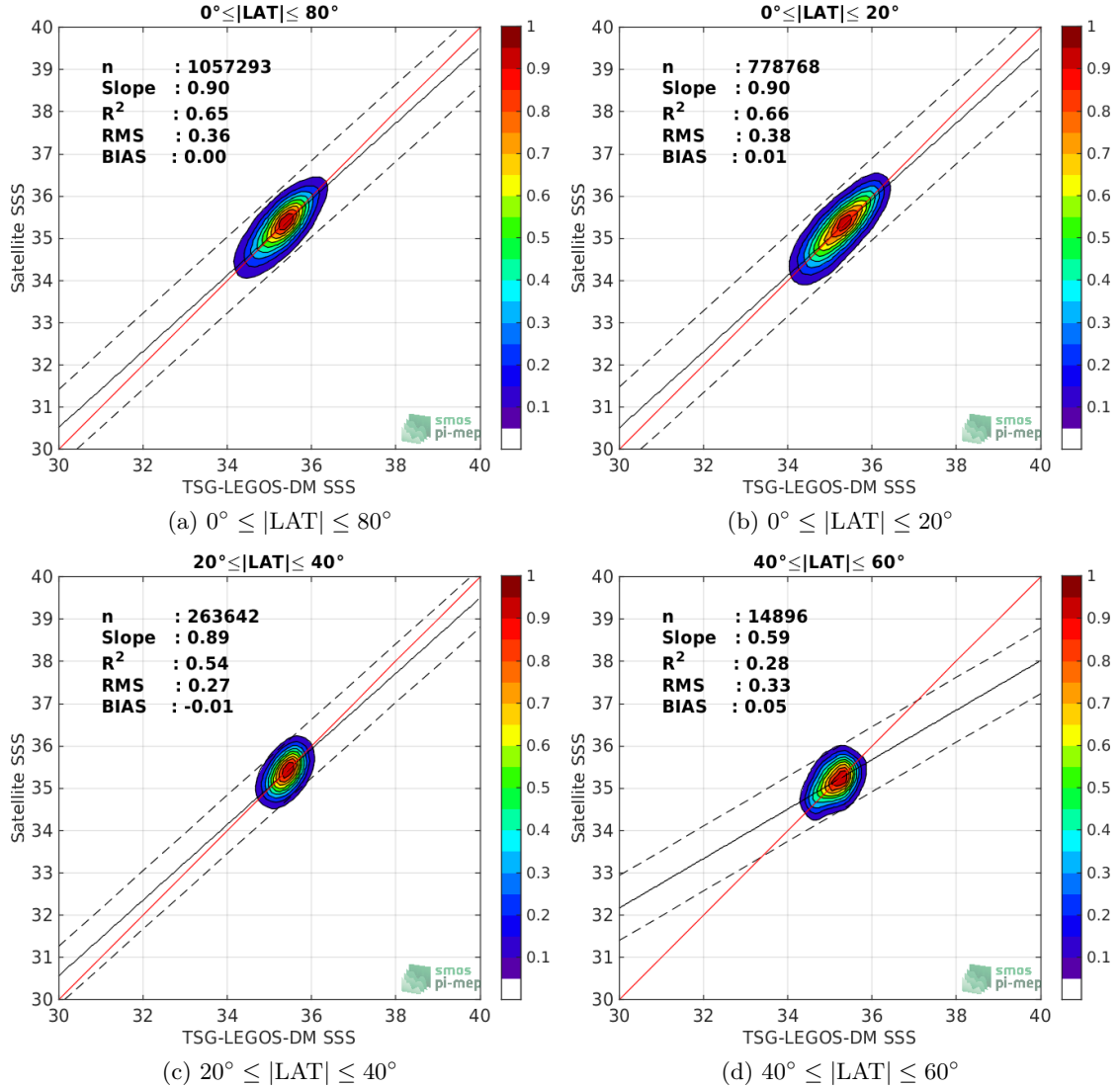
Figure 9: Contour maps of the concentration of SMOS-L3-CATDS-CECOS-LOCEAN-V4-9DAYS-25KM SSS (y-axis) versus TSG-LEGOS-DM SSS (x-axis) at match-up pairs for different latitude bands. For each plot, the red line shows x=y . The black thin and dashed lines indicate a linear fit through the data cloud and the \pm 95\% confidence levels, respectively. The number match-up pairs n , the slope and R^2 coefficient of the linear fit, the root mean square (RMS) and the mean bias between satellite and in situ data are indicated for each latitude band in each plots.
