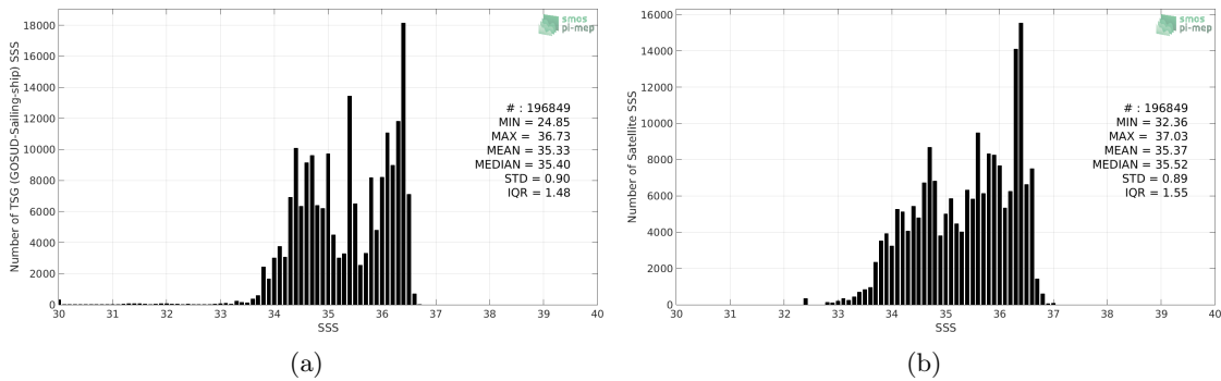
Figure 2: Histograms of SSS from TSG (GOSUD-Sailing-ship) (a) and SMOS SSS L3 v4 - 9 Days (CATDS-CECOS-LOCEAN) (b) considering all match-up pairs per bins of 0.1 over the South Pacific Ocean Pi-MEP region and for the full satellite product period.
