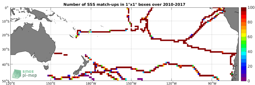
Figure 4: Number of SSS match-ups between TSG (GOSUD-Sailing-ship) SSS and the SMOS SSS L3 v4 - 9 Days (CATDS-CECOS-LOCEAN) SSS product for the South Pacific Ocean Pi-MEP region over 1^\circ \times 1^\circ boxes and for the full satellite product period.
