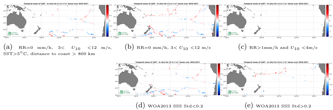
Figure 12: Temporal mean gridded over spatial boxes of size 1^\circ \times 1^\circ of \Delta SSS (SMOS SSS L3 v4 - 9 Days (CATDS-CECOS-LOCEAN) - TSG (GOSUD-Sailing-ship)) for 5 different subdatasets corresponding to:RR=0 mm/h, 3 < U_{10} < 12 m/s, SST>5°C, distance to coast > 800 km (a), RR=0 mm/h, 3 < U_{10} < 12 m/s (b), RR>1mm/h and U_{10} < 4 m/s (c), WOA2013 SSS Std<0.2 (d), WOA2013 SSS Std>0.2 (e).
