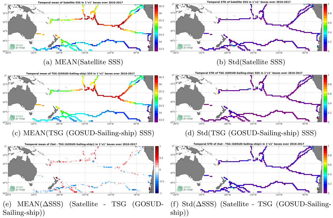
Figure 6: Temporal mean (left) and Std (right) of SSS from SMOS SSS L3 v4 - 9 Days (CATDS-CECOS-LOCEAN) (top), TSG (GOSUD-Sailing-ship) (middle), and of \Delta SSS (Satellite - TSG (GOSUD-Sailing-ship)). Only match-up pairs are used to generate these maps.
