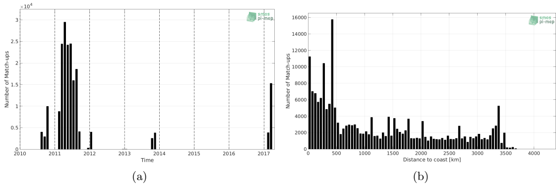
Figure 1: Number of match-ups between TSG (GOSUD-Sailing-ship) and SMOS SSS L3 v4 - 9 Days (CATDS-CECOS-LOCEAN) SSS as a function of time (a) and as function of the distance to coast (b) over the South Pacific Ocean Pi-MEP region and for the full satellite product period.
