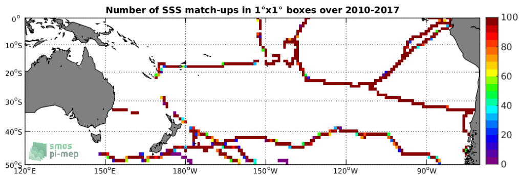
Figure 4: Number of SSS match-ups between TSG-GOSUD-Sailing-ship SSS and the SMOS-L3-CATDS-CECOS-LOCEAN-V4-9DAYS-25KM SSS product for the South Pacific Ocean Pi-MEP region over 1^\circ \times 1^\circ boxes and for the full satellite product period.
