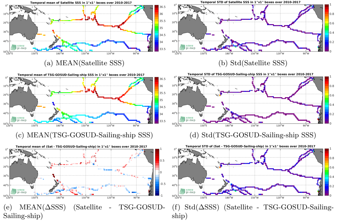
Figure 6: Temporal mean (left) and Std (right) of SSS from SMOS-L3-CATDS-CECOS-LOCEAN-V4-9DAYS-25KM (top), TSG-GOSUD-Sailing-ship (middle), and of \Delta SSS (Satellite - TSG-GOSUD-Sailing-ship). Only match-up pairs are used to generate these maps.
