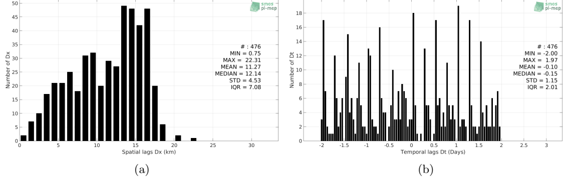
Figure 5: Histograms of the spatial (a) and temporal (b) lags between the time of the Sea mammals measurements and the date of the corresponding SMOS SSS L3 v4 - 9 Days (CATDS-CECOS-LOCEAN) SSS product.
