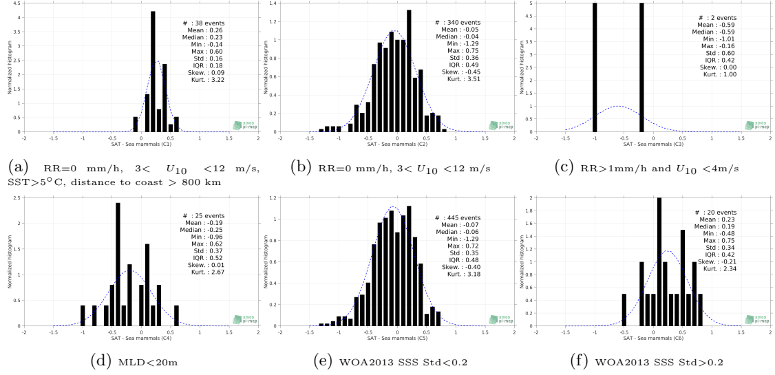
Figure 13: Normalized histogram of \Delta SSS (SMOS SSS L3 v4 - 9 Days (CATDS-CECOS-LOCEAN) - Sea mammals) for 6 different subdatasets corresponding to: RR=0 mm/h, 3 < U_{10} < 12 m/s, SST>5°C, distance to coast > 800 km (a), RR=0 mm/h, 3 < U_{10} < 12 m/s (b), RR>1mm/h and U_{10} < 4 m/s (c), MLD<20m (d), WOA2013 SSS Std<0.2 (e), WOA2013 SSS Std>0.2 (f).
