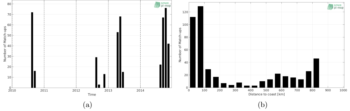
Figure 1: Number of match-ups between Sea mammals and SMOS SSS L3 v4 - 9 Days (CATDS-CECOS-LOCEAN) SSS as a function of time (a) and as function of the distance to coast (b) over the South Pacific Ocean Pi-MEP region and for the full satellite product period.
