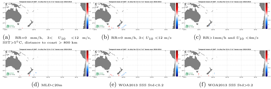
Figure 12: Temporal mean gridded over spatial boxes of size 1^{\circ}\times 1^{\circ} of \Delta\text{SSS} (SMOS SSS L3 v4 - 9 Days (CATDS-CECOS-LOCEAN) - Sea mammals) for 6 different subdatasets corresponding to:RR=0 mm/h, 3 < U_{10} < 12 m/s, SST >5^{\circ}\text{C} , distance to coast > 800 km (a), RR=0 mm/h, 3 < U_{10} < 12 m/s (b), RR >1\text{mm/h} and U_{10} < 4\text{m/s} (c),MLD <20\text{m} (d),WOA2013 SSS Std <0.2 (e),WOA2013 SSS Std >0.2 (f).
