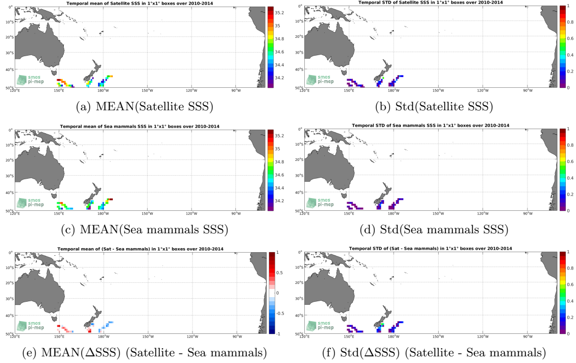
Figure 6: Temporal mean (left) and Std (right) of SSS from SMOS SSS L3 v4 - 9 Days (CATDS-CECOS-LOCEAN) (top), Sea mammals (middle), and of \Delta SSS (Satellite - Sea mammals). Only match-up pairs are used to generate these maps.
