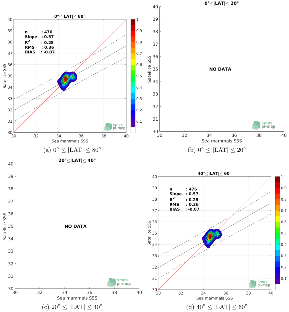
Figure 9: Contour maps of the concentration of SMOS SSS L3 v4 - 9 Days (CATDS-CECOS-LOCEAN) SSS (y-axis) versus Sea mammals SSS (x-axis) at match-up pairs for different latitude bands. For each plot, the red line shows x=y . The black thin and dashed lines indicate a linear fit through the data cloud and the \pm 95\% confidence levels, respectively. The number match-up pairs n , the slope and R^2 coefficient of the linear fit, the root mean square (RMS) and the mean bias between satellite and in situ data are indicated for each latitude band in each plots.
