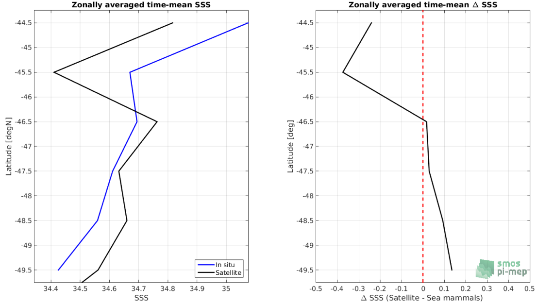
Figure 8: Left panel: Zonal mean SSS from SMOS SSS L3 v4 - 9 Days (CATDS-CECOS-LOCEAN) satellite product (black) and from Sea mammals (blue). Right panel: Zonal mean of \Delta SSS (Satellite - Sea mammals) for all the collected Pi-MEP match-up pairs estimated over the full satellite product period.
