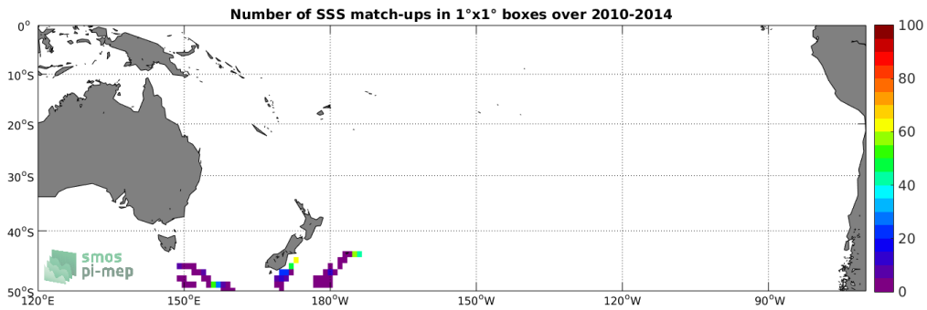
Figure 4: Number of SSS match-ups between Sea mammals SSS and the SMOS SSS L3 v4 - 9 Days (CATDS-CECOS-LOCEAN) SSS product for the South Pacific Ocean Pi-MEP region over 1°x1° boxes and for the full satellite product period.
