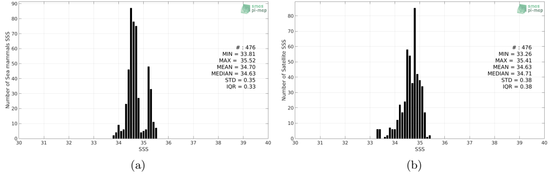
Figure 2: Histograms of SSS from Sea mammals (a) and SMOS SSS L3 v4 - 9 Days (CATDS-CECOS-LOCEAN) (b) considering all match-up pairs per bins of 0.1 over the South Pacific Ocean Pi-MEP region and for the full satellite product period.
