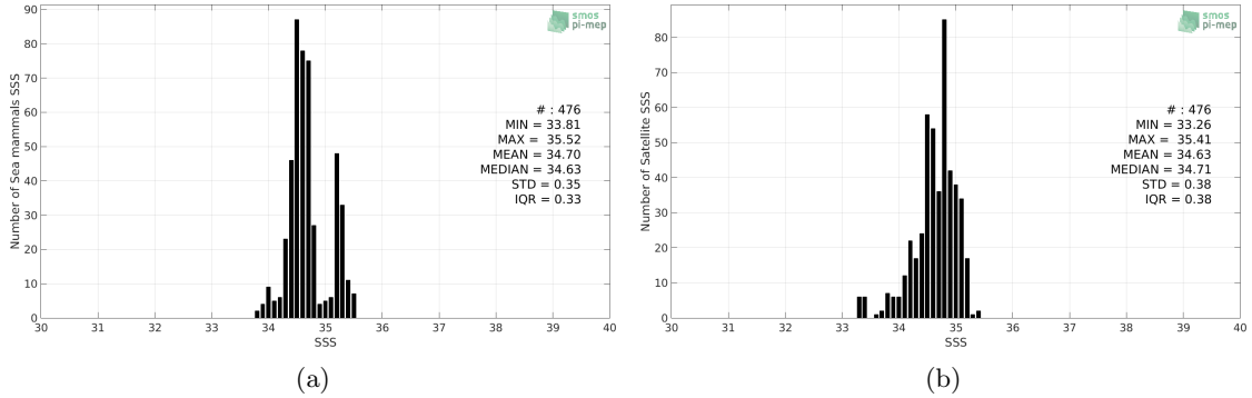
Figure 2: Histograms of SSS from Sea mammals (a) and SMOS-L3-CATDS-CECOS-LOCEAN-V4-9DAYS-25KM (b) considering all match-up pairs per bins of 0.1 over the South Pacific Ocean Pi-MEP region and for the full satellite product period.
