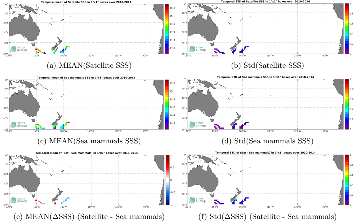
Figure 6: Temporal mean (left) and Std (right) of SSS from SMOS-L3-CATDS-CECOS-LOCEAN-V4-9DAYS-25KM (top), Sea mammals (middle), and of \Delta SSS (Satellite - Sea mammals). Only match-up pairs are used to generate these maps.
