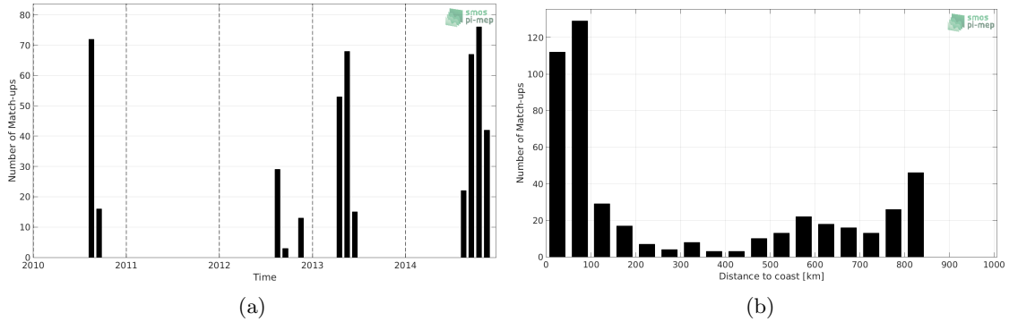
Figure 1: Number of match-ups between Sea mammals and SMOS-L3-CATDS-CECOS-LOCEAN-V4-9DAYS-25KM SSS as a function of time (a) and as function of the distance to coast (b) over the South Pacific Ocean Pi-MEP region and for the full satellite product period.
