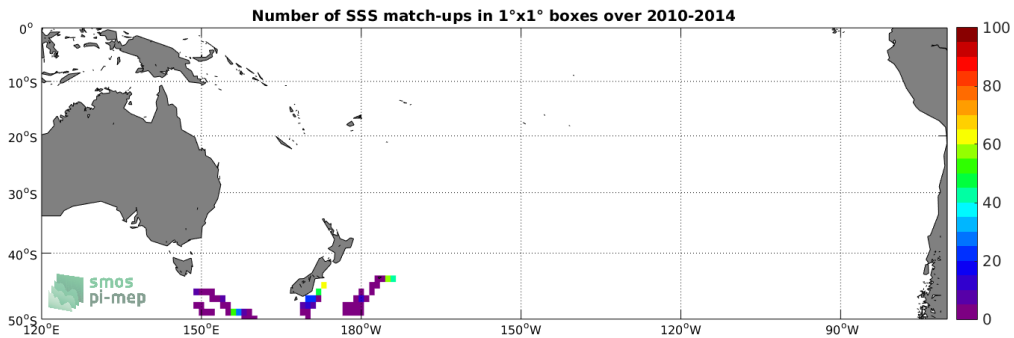
Figure 4: Number of SSS match-ups between Sea mammals SSS and the SMOS-L3-CATDS-CECOS-LOCEAN-V4-9DAYS-25KM SSS product for the South Pacific Ocean Pi-MEP region over 1^\circ \times 1^\circ boxes and for the full satellite product period.
