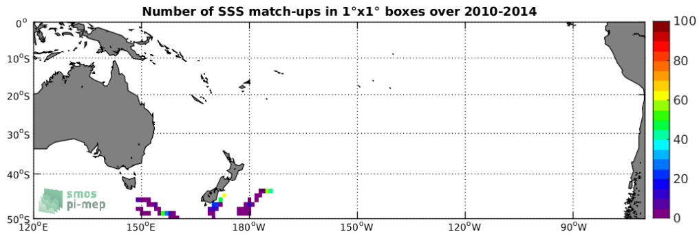
Figure 4: Number of SSS match-ups between Sea mammals SSS and the SMOS-L3-CATDS-CECOS-LOCEAN-V4-9DAYS-25KM SSS product for the South Pacific Ocean Pi-MEP region over 1°x1° boxes and for the full satellite product period.
