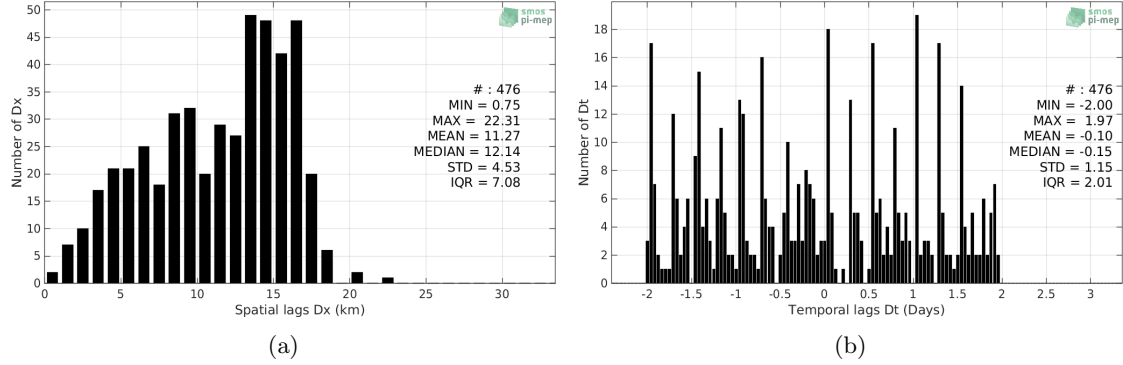
Figure 5: Histograms of the spatial (a) and temporal (b) lags between the time of the Sea mammals measurements and the date of the corresponding SMOS-L3-CATDS-CECOS-LOCEAN-V4-9DAYS-25KM SSS product.
