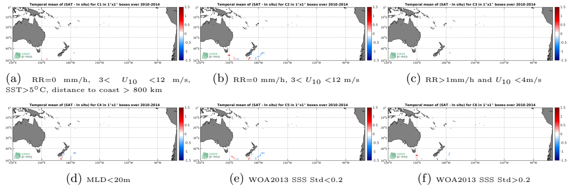
Figure 12: Temporal mean gridded over spatial boxes of size 1^\circ \times 1^\circ of \Delta SSS (SMOS-L3-CATDS-CECOS-LOCEAN-V4-9DAYS-25KM - Sea mammals) for 6 different subdatasets corresponding to: RR=0 mm/h, 3 < U_{10} < 12 m/s, SST > 5^\circ C , distance to coast > 800 km (a), RR=0 mm/h, 3 < U_{10} < 12 m/s (b), RR > 1 mm/h and U_{10} < 4 m/s (c), MLD < 20 m (d), WOA2013 SSS Std < 0.2 (e), WOA2013 SSS Std > 0.2 (f).
