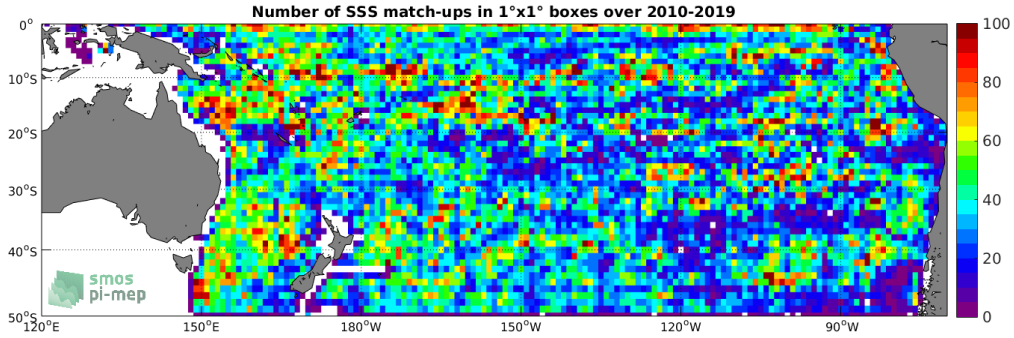
Figure 4: Number of SSS match-ups between Argo SSS and the SMOS SSS L3 v4 - 9 Days (CATDS-CECOS-LOCEAN) SSS product for the South Pacific Ocean Pi-MEP region over 1^\circ \times 1^\circ boxes and for the full satellite product period.
