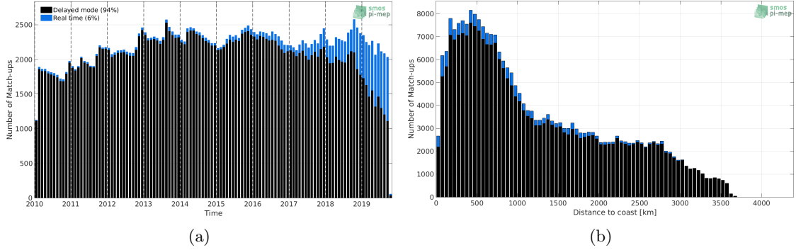
Figure 1: Number of match-ups between Argo and SMOS SSS L3 v4 - 9 Days (CATDS-CECOS-LOCEAN) SSS as a function of time (a) and as function of the distance to coast (b) over the South Pacific Ocean Pi-MEP region and for the full satellite product period.
