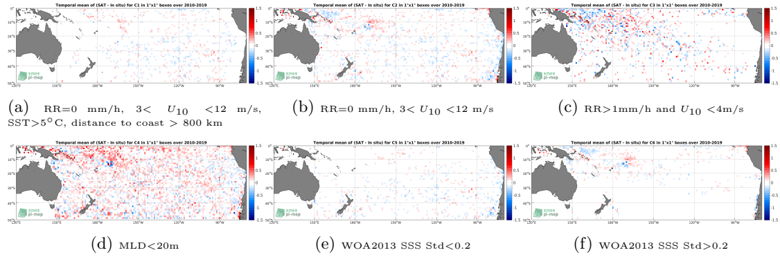
Figure 12: Temporal mean gridded over spatial boxes of size 1^\circ \times 1^\circ of \Delta SSS (SMOS SSS L3 v4 - 9 Days (CATDS-CECOS-LOCEAN) - Argo) for 6 different subdatasets corresponding to: RR=0 mm/h, 3 < U_{10} < 12 m/s, SST > 5^\circ C , distance to coast > 800 km (a), RR=0 mm/h, 3 < U_{10} < 12 m/s (b), RR > 1 mm/h and U_{10} < 4 m/s (c), MLD < 20 m (d), WOA2013 SSS Std < 0.2 (e), WOA2013 SSS Std > 0.2 (f).
