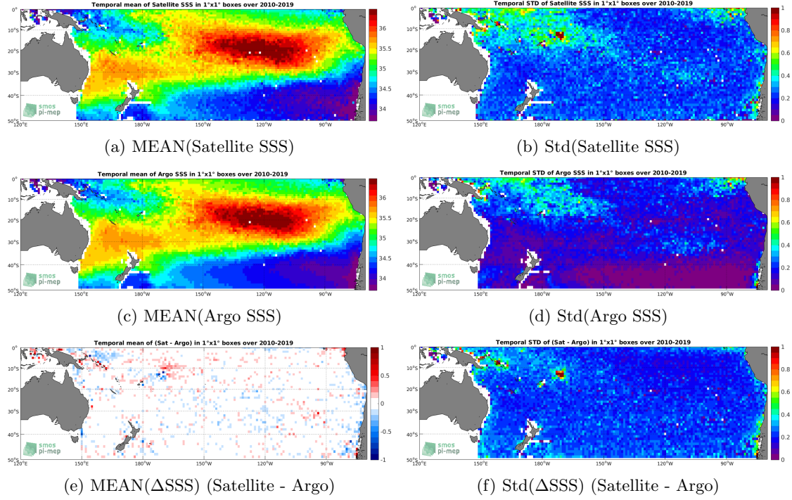
Figure 6: Temporal mean (left) and Std (right) of SSS from SMOS SSS L3 v4 - 9 Days (CATDS-CECOS-LOCEAN) (top), Argo (middle), and of \Delta SSS (Satellite - Argo). Only match-up pairs are used to generate these maps.
