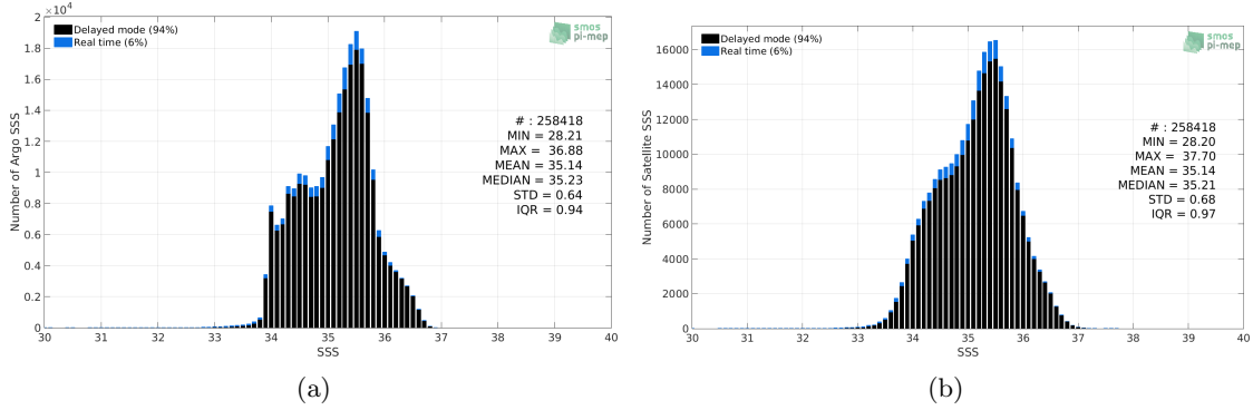
Figure 2: Histograms of SSS from Argo (a) and SMOS SSS L3 v4 - 9 Days (CATDS-CECOS-LOCEAN) (b) considering all match-up pairs per bins of 0.1 over the South Pacific Ocean Pi-MEP region and for the full satellite product period.
