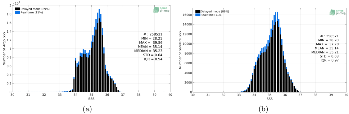
Figure 2: Histograms of SSS from Argo (a) and SMOS-L3-CATDS-CECOS-LOCEAN-V4-9DAYS-25KM (b) considering all match-up pairs per bins of 0.1 over the South Pacific Ocean Pi-MEP region and for the full satellite product period.
