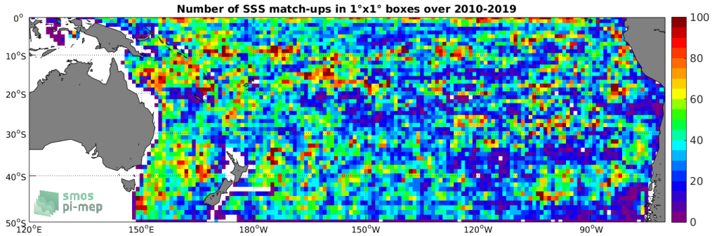
Figure 4: Number of SSS match-ups between Argo SSS and the SMOS-L3-CATDS-CECOS-LOCEAN-V4-9DAYS-25KM SSS product for the South Pacific Ocean Pi-MEP region over 1^\circ \times 1^\circ boxes and for the full satellite product period.
