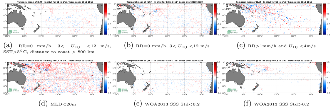
Figure 12: Temporal mean gridded over spatial boxes of size 1^\circ \times 1^\circ of \Delta SSS (SMOS-L3-CATDS-CECOS-LOCEAN-V4-9DAYS-25KM - Argo) for 6 different subdatasets corresponding to: RR=0 mm/h, 3 < U_{10} < 12 m/s, SST > 5^\circ C , distance to coast > 800 km (a), RR=0 mm/h, 3 < U_{10} < 12 m/s (b), RR > 1 mm/h and U_{10} < 4 m/s (c), MLD < 20 m (d), WOA2013 SSS Std < 0.2 (e), WOA2013 SSS Std > 0.2 (f).
