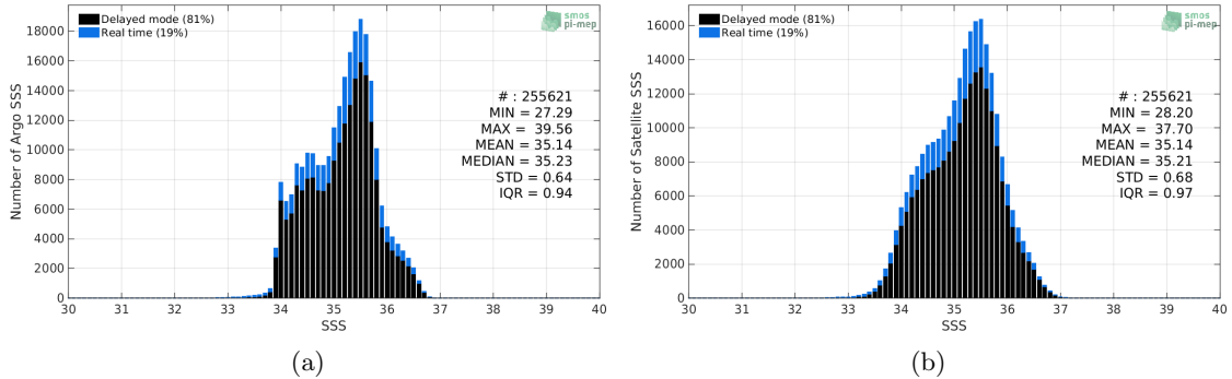
Figure 2: Histograms of SSS from Argo (a) and SMOS-L3-CATDS-CECOS-LOCEAN-V4-9DAYS-25KM (b) considering all match-up pairs per bins of 0.1 over the South Pacific Ocean Pi-MEP region and for the full satellite product period.
