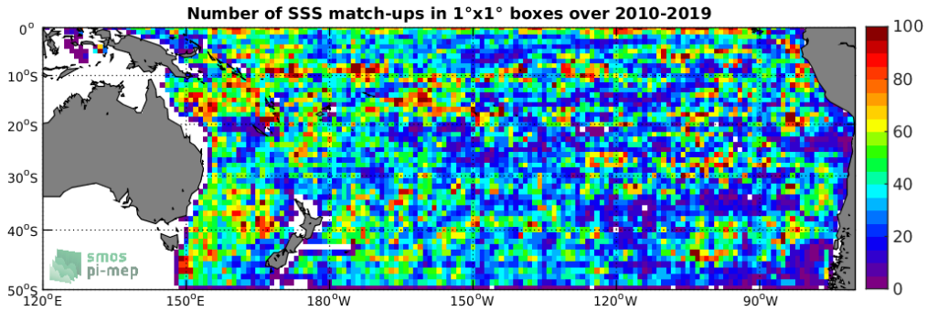
Figure 4: Number of SSS match-ups between Argo SSS and the SMOS-L3-CATDS-CECOS-LOCEAN-V4-9DAYS-25KM SSS product for the South Pacific Ocean Pi-MEP region over 1°x1° boxes and for the full satellite product period.
