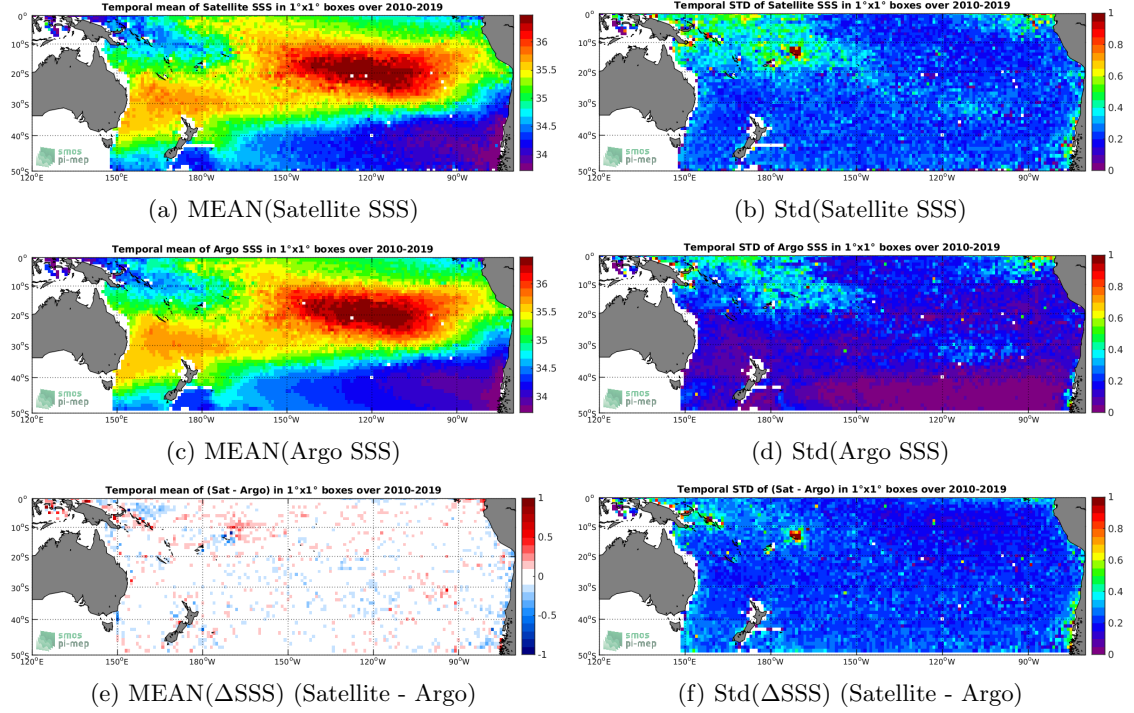
Figure 6: Temporal mean (left) and Std (right) of SSS from SMOS-L3-CATDS-CECOS-LOCEAN-V4-9DAYS-25KM (top), Argo (middle), and of \Delta SSS (Satellite - Argo). Only match-up pairs are used to generate these maps.
