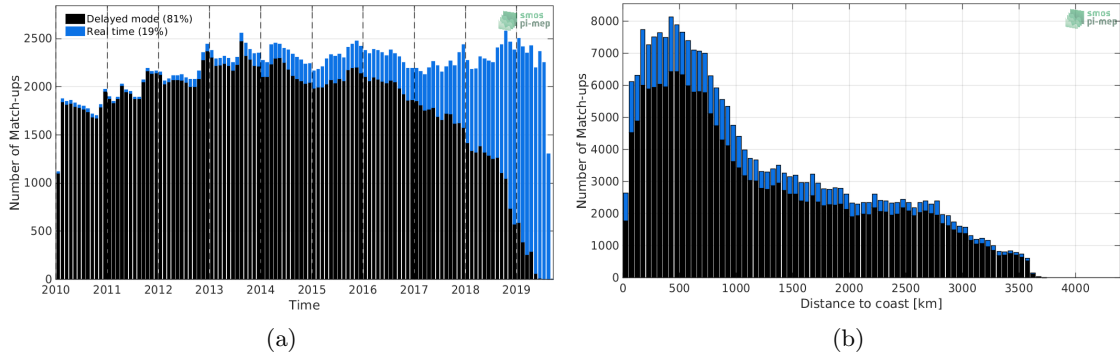
Figure 1: Number of match-ups between Argo and SMOS-L3-CATDS-CECOS-LOCEAN-V4-9DAYS-25KM SSS as a function of time (a) and as function of the distance to coast (b) over the South Pacific Ocean Pi-MEP region and for the full satellite product period.
