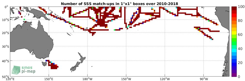
Figure 4: Number of SSS match-ups between TSG (SAMOS) SSS and the SMOS SSS L3 v4 - 18 Days (CATDS-CECOS-LOCEAN) SSS product for the South Pacific Ocean Pi-MEP region over 1^\circ \times 1^\circ boxes and for the full satellite product period.
