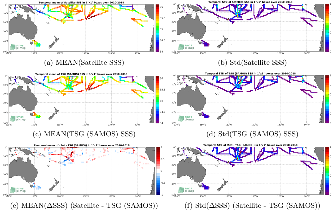
Figure 6: Temporal mean (left) and Std (right) of SSS from SMOS SSS L3 v4 - 18 Days (CATDS-CECOS-LOCEAN) (top), TSG (SAMOS) (middle), and of \Delta SSS (Satellite - TSG (SAMOS)). Only match-up pairs are used to generate these maps.
