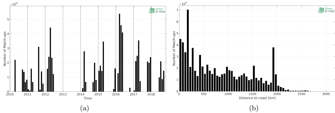
Figure 1: Number of match-ups between TSG (SAMOS) and SMOS SSS L3 v4 - 18 Days (CATDS-CECOS-LOCEAN) SSS as a function of time (a) and as function of the distance to coast (b) over the South Pacific Ocean Pi-MEP region and for the full satellite product period.
