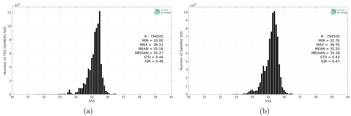
Figure 2: Histograms of SSS from TSG (SAMOS) (a) and SMOS SSS L3 v4 - 18 Days (CATDS-CECOS-LOCEAN) (b) considering all match-up pairs per bins of 0.1 over the South Pacific Ocean Pi-MEP region and for the full satellite product period.
