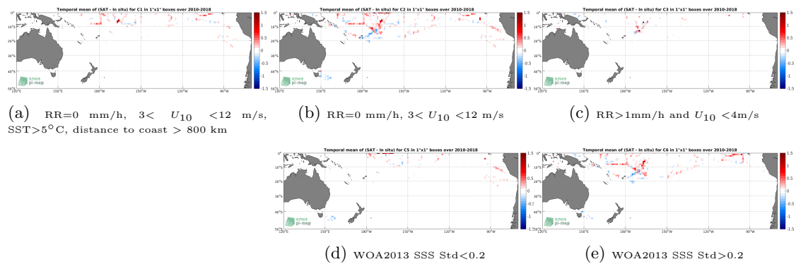
Figure 12: Temporal mean gridded over spatial boxes of size 1^\circ \times 1^\circ of \Delta SSS (SMOS SSS L3 v4 - 18 Days (CATDS-CECOS-LOCEAN) - TSG (SAMOS)) for 5 different subdatasets corresponding to: RR=0 mm/h, 3 < U_{10} < 12 m/s, SST > 5°C, distance to coast > 800 km (a), RR=0 mm/h, 3 < U_{10} < 12 m/s (b), RR > 1mm/h and U_{10} < 4 m/s (c), WOA2013 SSS Std < 0.2 (d), WOA2013 SSS Std > 0.2 (e).
