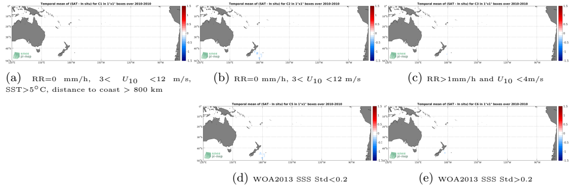
Figure 12: Temporal mean gridded over spatial boxes of size 1^{\circ}\times 1^{\circ} of \Delta\text{SSS} (SMOS SSS L3 v4 - 18 Days (CATDS-CECOS-LOCEAN) - TSG (Polarstern)) for 5 different subdatasets corresponding to:RR=0 mm/h, 3 < U_{10} < 12 m/s, SST >5^{\circ}\text{C} , distance to coast > 800 km (a), RR=0 mm/h, 3 < U_{10} < 12 m/s (b), RR >1 mm/h and U_{10} < 4 m/s (c), WOA2013 SSS Std <0.2 (d), WOA2013 SSS Std >0.2 (e).
