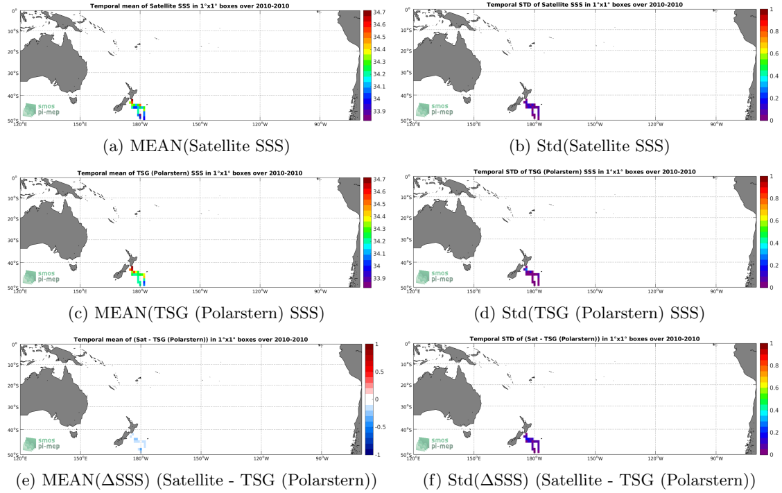
Figure 6: Temporal mean (left) and Std (right) of SSS from SMOS SSS L3 v4 - 18 Days (CATDS-CECOS-LOCEAN) (top), TSG (Polarstern) (middle), and of \Delta SSS (Satellite - TSG (Polarstern)). Only match-up pairs are used to generate these maps.
