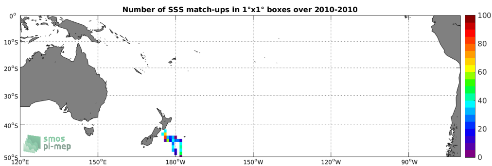
Figure 4: Number of SSS match-ups between TSG (Polarstern) SSS and the SMOS SSS L3 v4 - 18 Days (CATDS-CECOS-LOCEAN) SSS product for the South Pacific Ocean Pi-MEP region over 1^\circ \times 1^\circ boxes and for the full satellite product period.
