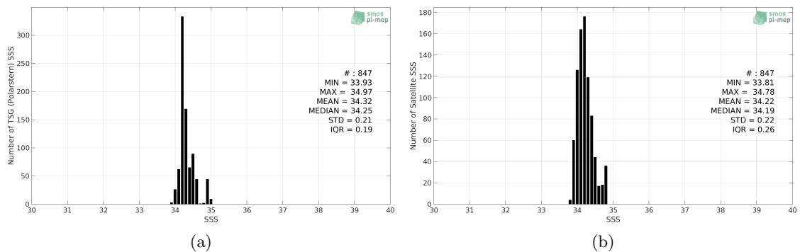
Figure 2: Histograms of SSS from TSG (Polarstern) (a) and SMOS SSS L3 v4 - 18 Days (CATDS-CECOS-LOCEAN) (b) considering all match-up pairs per bins of 0.1 over the South Pacific Ocean Pi-MEP region and for the full satellite product period.
