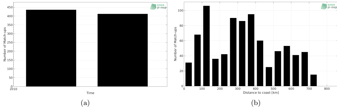
Figure 1: Number of match-ups between TSG (Polarstern) and SMOS SSS L3 v4 - 18 Days (CATDS-CECOS-LOCEAN) SSS as a function of time (a) and as function of the distance to coast (b) over the South Pacific Ocean Pi-MEP region and for the full satellite product period.
