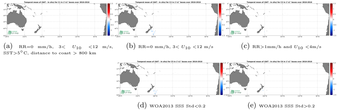
Figure 12: Temporal mean gridded over spatial boxes of size 1^{\circ}\times 1^{\circ} of \Delta\text{SSS} (SMOS-L3-CATDS-CECOS-LOCEAN-V4-18DAYS-25KM - TSG-POLARSTERN) for 5 different subdatasets corresponding to:RR=0 mm/h, 3 < U_{10} < 12 m/s, SST > 5^{\circ}\text{C} , distance to coast > 800 km (a), RR=0 mm/h, 3 < U_{10} < 12 m/s (b), RR > 1 mm/h and U_{10} < 4 m/s (c), WOA2013 SSS Std < 0.2 (d), WOA2013 SSS Std > 0.2 (e).
