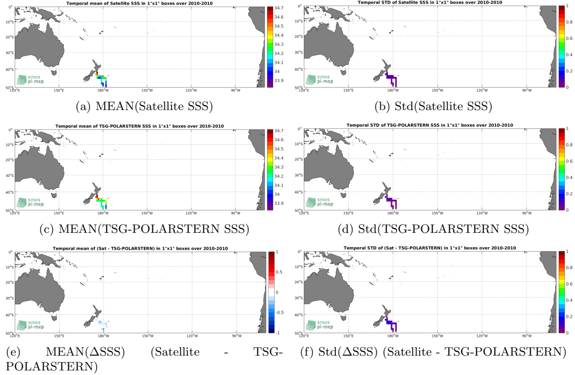
Figure 6: Temporal mean (left) and Std (right) of SSS from SMOS-L3-CATDS-CECOS-LOCEAN-V4-18DAYS-25KM (top), TSG-POLARSTERN (middle), and of \Delta SSS (Satellite - TSG-POLARSTERN). Only match-up pairs are used to generate these maps.
