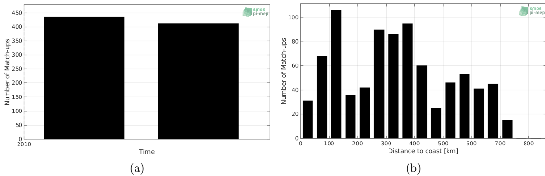
Figure 1: Number of match-ups between TSG-POLARSTERN and SMOS-L3-CATDS-CECOS-LOCEAN-V4-18DAYS-25KM SSS as a function of time (a) and as function of the distance to coast (b) over the South Pacific Ocean Pi-MEP region and for the full satellite product period.
