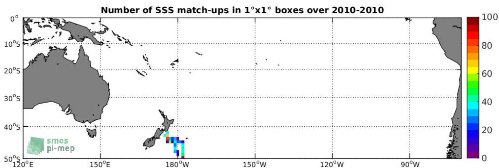
Figure 4: Number of SSS match-ups between TSG-POLARSTERN SSS and the SMOS-L3-CATDS-CECOS-LOCEAN-V4-18DAYS-25KM SSS product for the South Pacific Ocean Pi-MEP region over 1^\circ \times 1^\circ boxes and for the full satellite product period.
