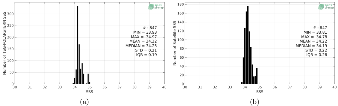
Figure 2: Histograms of SSS from TSG-POLARSTERN (a) and SMOS-L3-CATDS-CECOS-LOCEAN-V4-18DAYS-25KM (b) considering all match-up pairs per bins of 0.1 over the South Pacific Ocean Pi-MEP region and for the full satellite product period.
