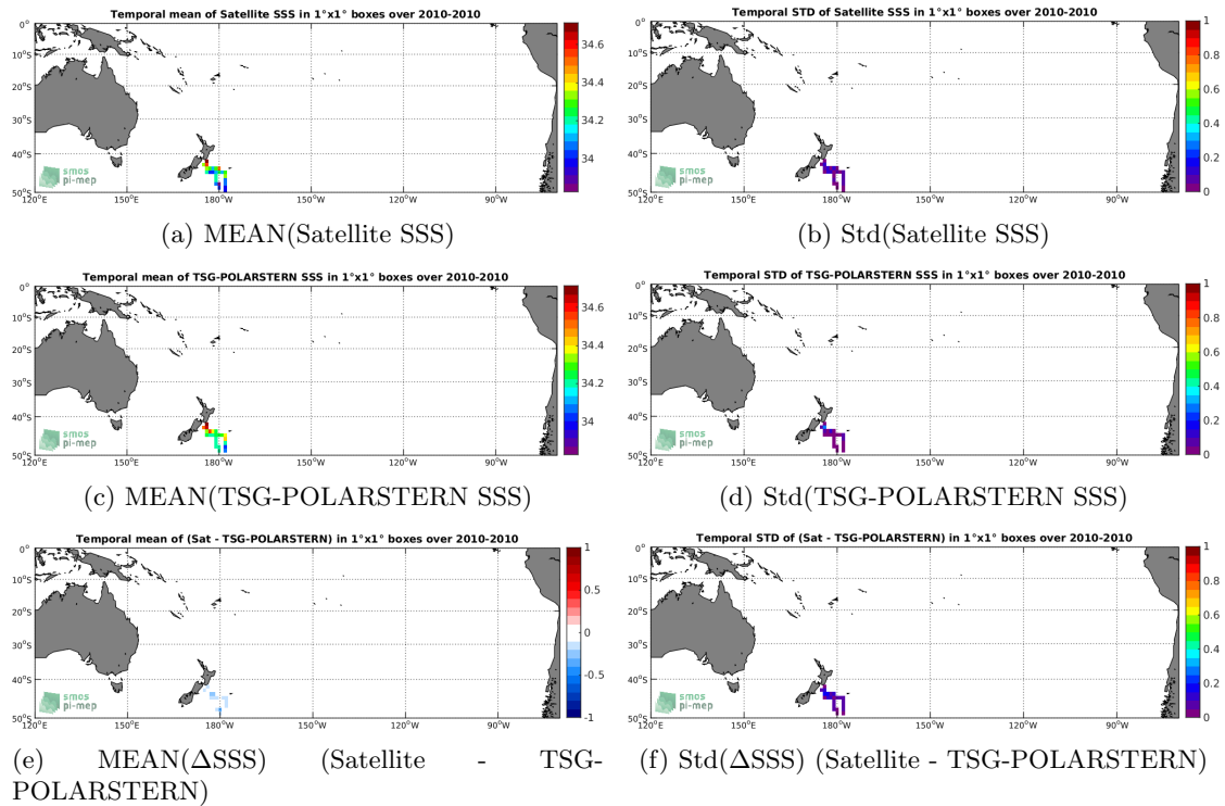
Figure 6: Temporal mean (left) and Std (right) of SSS from SMOS-L3-CATDS-CECOS-LOCEAN-V4-18DAYS-25KM (top), TSG-POLARSTERN (middle), and of \Delta SSS (Satellite - TSG-POLARSTERN). Only match-up pairs are used to generate these maps.
