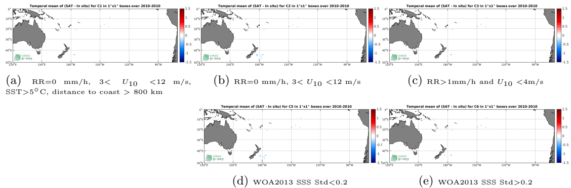
Figure 12: Temporal mean gridded over spatial boxes of size 1^\circ \times 1^\circ of \Delta SSS (SMOS-L3-CATDS-CECOS-LOCEAN-V4-18DAYS-25KM - TSG-POLARSTERN) for 5 different subdatasets corresponding to:RR=0 mm/h, 3 < U_{10} < 12 m/s, SST >5^\circ C, distance to coast > 800 km (a), RR=0 mm/h, 3 < U_{10} < 12 m/s (b), RR >1 mm/h and U_{10} < 4 m/s (c), WOA2013 SSS Std <0.2 (d), WOA2013 SSS Std >0.2 (e).
