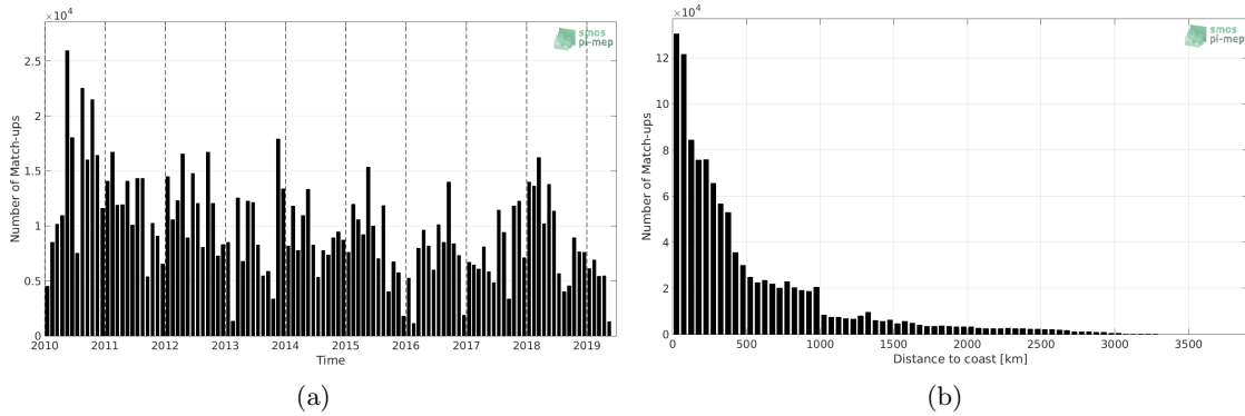
Figure 1: Number of match-ups between TSG (LEGOS-DM) and SMOS SSS L3 v4 - 18 Days (CATDS-CECOS-LOCEAN) SSS as a function of time (a) and as function of the distance to coast (b) over the South Pacific Ocean Pi-MEP region and for the full satellite product period.
