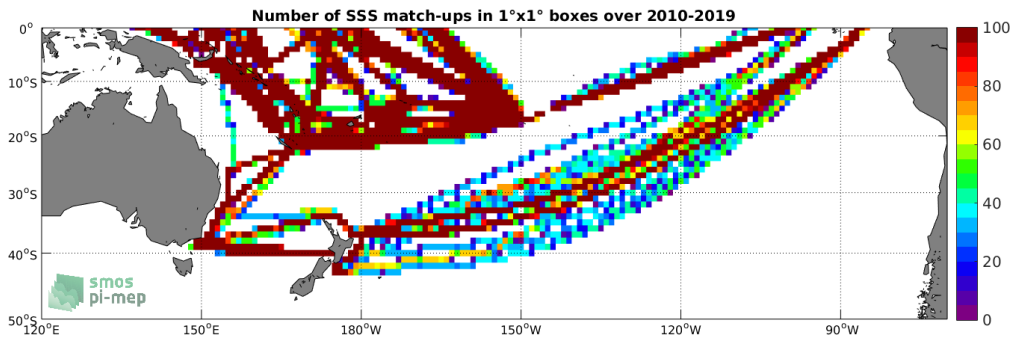
Figure 4: Number of SSS match-ups between TSG (LEGOS-DM) SSS and the SMOS SSS L3 v4 - 18 Days (CATDS-CECOS-LOCEAN) SSS product for the South Pacific Ocean Pi-MEP region over 1^\circ \times 1^\circ boxes and for the full satellite product period.
