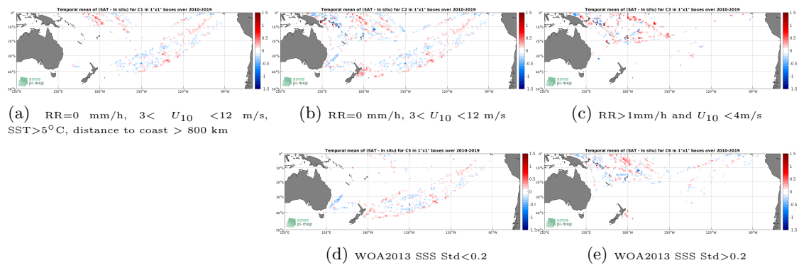
Figure 12: Temporal mean gridded over spatial boxes of size 1^\circ \times 1^\circ of \Delta SSS (SMOS SSS L3 v4 - 18 Days (CATDS-CECOS-LOCEAN) - TSG (LEGOS-DM)) for 5 different subdatasets corresponding to:RR=0 mm/h, 3 < U_{10} < 12 m/s, SST >5^\circ C, distance to coast > 800 km (a), RR=0 mm/h, 3 < U_{10} < 12 m/s (b), RR >1 mm/h and U_{10} < 4 m/s (c), WOA2013 SSS Std <0.2 (d), WOA2013 SSS Std >0.2 (e).
