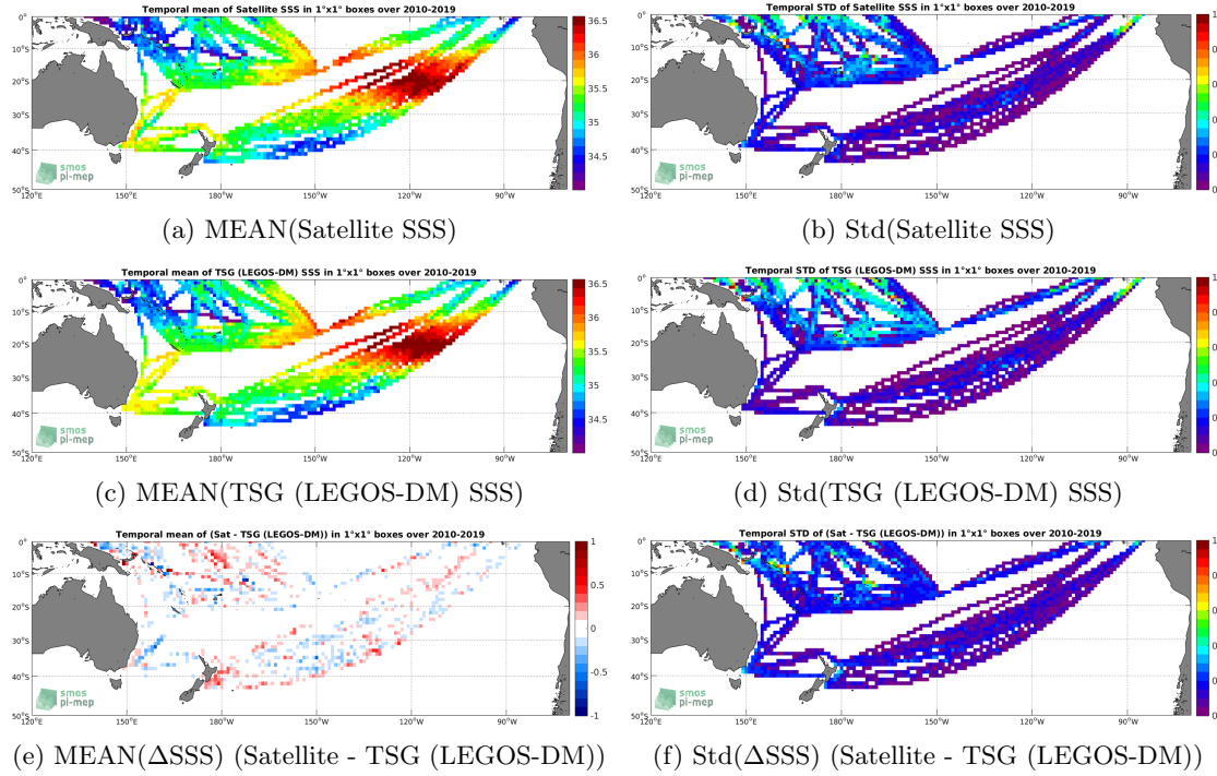
Figure 6: Temporal mean (left) and Std (right) of SSS from SMOS SSS L3 v4 - 18 Days (CATDS-CECOS-LOCEAN) (top), TSG (LEGOS-DM) (middle), and of \Delta SSS (Satellite - TSG (LEGOS-DM)). Only match-up pairs are used to generate these maps.
