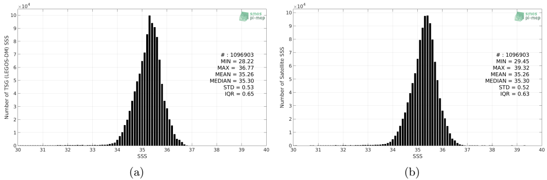
Figure 2: Histograms of SSS from TSG (LEGOS-DM) (a) and SMOS SSS L3 v4 - 18 Days (CATDS-CECOS-LOCEAN) (b) considering all match-up pairs per bins of 0.1 over the South Pacific Ocean Pi-MEP region and for the full satellite product period.
