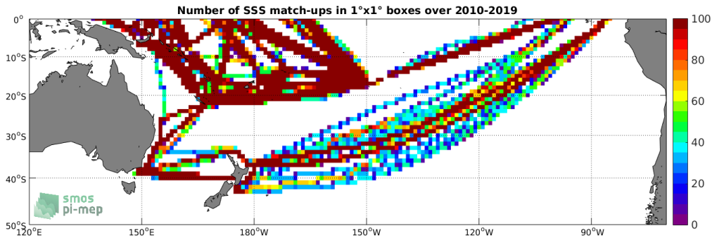
Figure 4: Number of SSS match-ups between TSG-LEGOS-DM SSS and the SMOS-L3-CATDS-CECOS-LOCEAN-V4-18DAYS-25KM SSS product for the South Pacific Ocean Pi-MEP region over 1°x1° boxes and for the full satellite product period.
