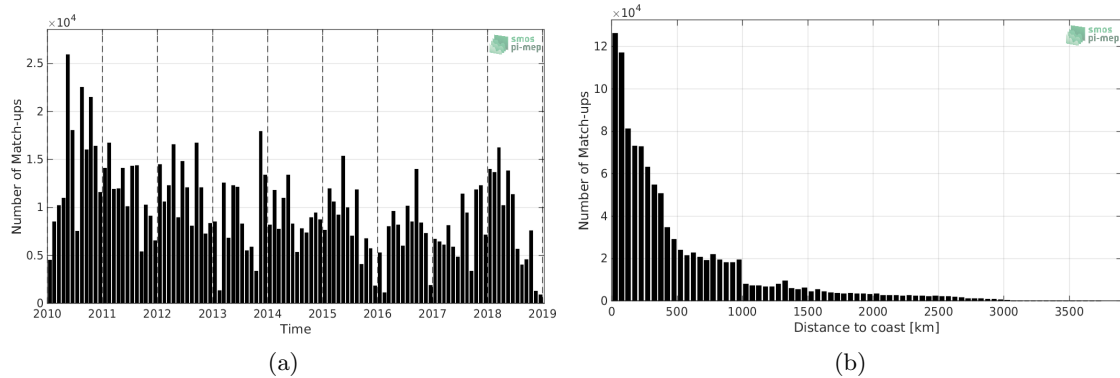
Figure 1: Number of match-ups between TSG-LEGOS-DM and SMOS-L3-CATDS-CECOS-LOCEAN-V4-18DAYS-25KM SSS as a function of time (a) and as function of the distance to coast (b) over the South Pacific Ocean Pi-MEP region and for the full satellite product period.
