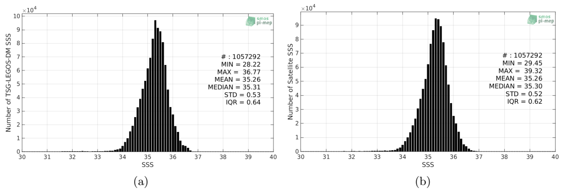
Figure 2: Histograms of SSS from TSG-LEGOS-DM (a) and SMOS-L3-CATDS-CECOS-LOCEAN-V4-18DAYS-25KM (b) considering all match-up pairs per bins of 0.1 over the South Pacific Ocean Pi-MEP region and for the full satellite product period.
