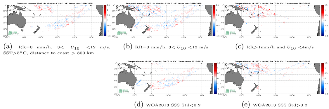
Figure 12: Temporal mean gridded over spatial boxes of size 1^\circ \times 1^\circ of \Delta SSS (SMOS-L3-CATDS-CECOS-LOCEAN-V4-18DAYS-25KM - TSG-LEGOS-DM) for 5 different subdatasets corresponding to:RR=0 mm/h, 3 < U_{10} < 12 m/s, SST >5^\circ C, distance to coast > 800 km (a), RR=0 mm/h, 3 < U_{10} < 12 m/s (b), RR >1 mm/h and U_{10} < 4 m/s (c), WOA2013 SSS Std <0.2 (d), WOA2013 SSS Std >0.2 (e).
