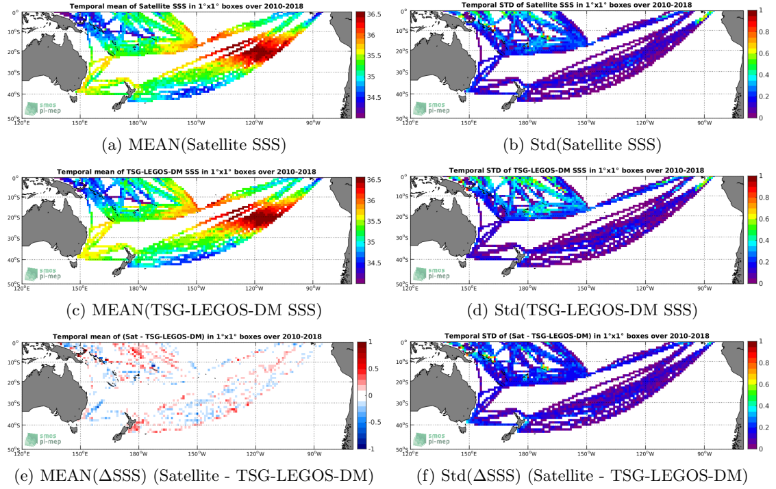
Figure 6: Temporal mean (left) and Std (right) of SSS from SMOS-L3-CATDS-CECOS-LOCEAN-V4-18DAYS-25KM (top), TSG-LEGOS-DM (middle), and of \Delta SSS (Satellite - TSG-LEGOS-DM). Only match-up pairs are used to generate these maps.
