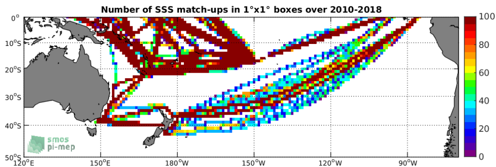
Figure 4: Number of SSS match-ups between TSG-LEGOS-DM SSS and the SMOS-L3-CATDS-CECOS-LOCEAN-V4-18DAYS-25KM SSS product for the South Pacific Ocean Pi-MEP region over 1^\circ \times 1^\circ boxes and for the full satellite product period.
