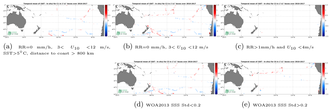
Figure 12: Temporal mean gridded over spatial boxes of size 1^\circ \times 1^\circ of \Delta\text{SSS} (SMOS SSS L3 v4 - 18 Days (CATDS-CECOS-LOCEAN) - TSG (GOSUD-Sailing-ship)) for 5 different subdatasets corresponding to:RR=0 mm/h, 3 < U_{10} < 12 m/s, SST>5°C, distance to coast > 800 km (a), RR=0 mm/h, 3 < U_{10} < 12 m/s (b), RR>1mm/h and U_{10} < 4 m/s (c), WOA2013 SSS Std<0.2 (d), WOA2013 SSS Std>0.2 (e).
