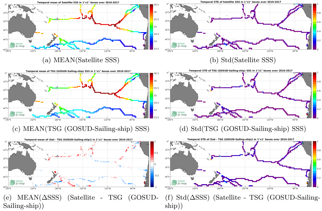
Figure 6: Temporal mean (left) and Std (right) of SSS from SMOS SSS L3 v4 - 18 Days (CATDS-CECOS-LOCEAN) (top), TSG (GOSUD-Sailing-ship) (middle), and of \Delta SSS (Satellite - TSG (GOSUD-Sailing-ship)). Only match-up pairs are used to generate these maps.
