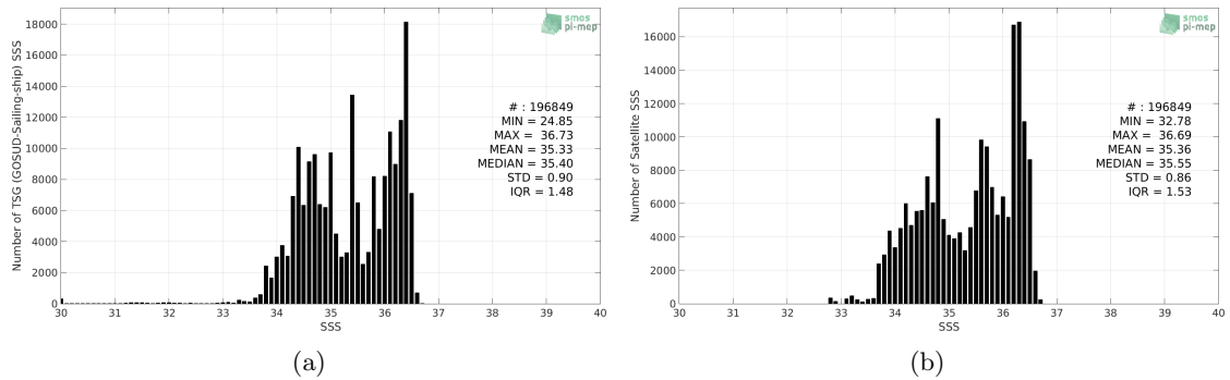
Figure 2: Histograms of SSS from TSG (GOSUD-Sailing-ship) (a) and SMOS SSS L3 v4 - 18 Days (CATDS-CECOS-LOCEAN) (b) considering all match-up pairs per bins of 0.1 over the South Pacific Ocean Pi-MEP region and for the full satellite product period.
