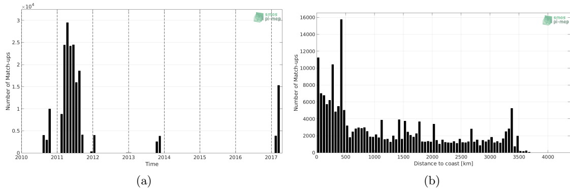
Figure 1: Number of match-ups between TSG (GOSUD-Sailing-ship) and SMOS SSS L3 v4 - 18 Days (CATDS-CECOS-LOCEAN) SSS as a function of time (a) and as function of the distance to coast (b) over the South Pacific Ocean Pi-MEP region and for the full satellite product period.
