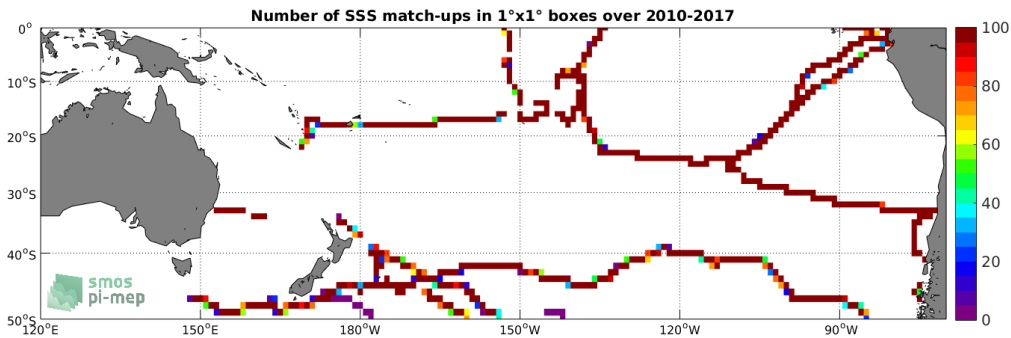
Figure 4: Number of SSS match-ups between TSG (GOSUD-Sailing-ship) SSS and the SMOS SSS L3 v4 - 18 Days (CATDS-CECOS-LOCEAN) SSS product for the South Pacific Ocean Pi-MEP region over 1^\circ \times 1^\circ boxes and for the full satellite product period.
