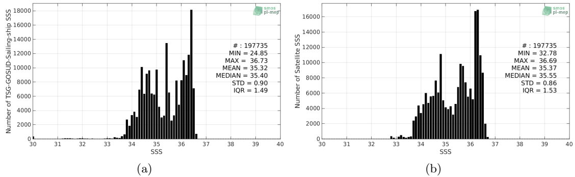
Figure 2: Histograms of SSS from TSG-GOSUD-Sailing-ship (a) and SMOS-L3-CATDS-CECOS-LOCEAN-V4-18DAYS-25KM (b) considering all match-up pairs per bins of 0.1 over the South Pacific Ocean Pi-MEP region and for the full satellite product period.
