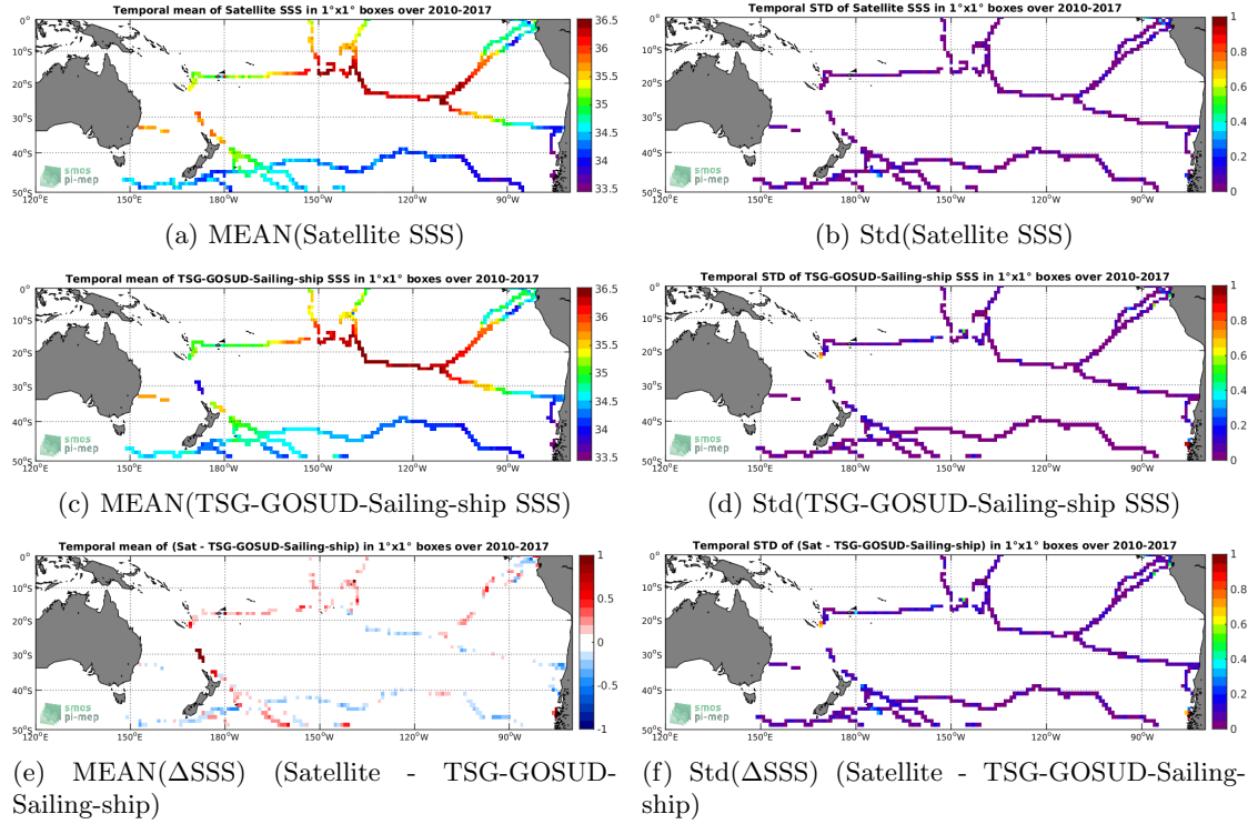
Figure 6: Temporal mean (left) and Std (right) of SSS from SMOS-L3-CATDS-CECOS-LOCEAN-V4-18DAYS-25KM (top), TSG-GOSUD-Sailing-ship (middle), and of \Delta SSS (Satellite - TSG-GOSUD-Sailing-ship). Only match-up pairs are used to generate these maps.
