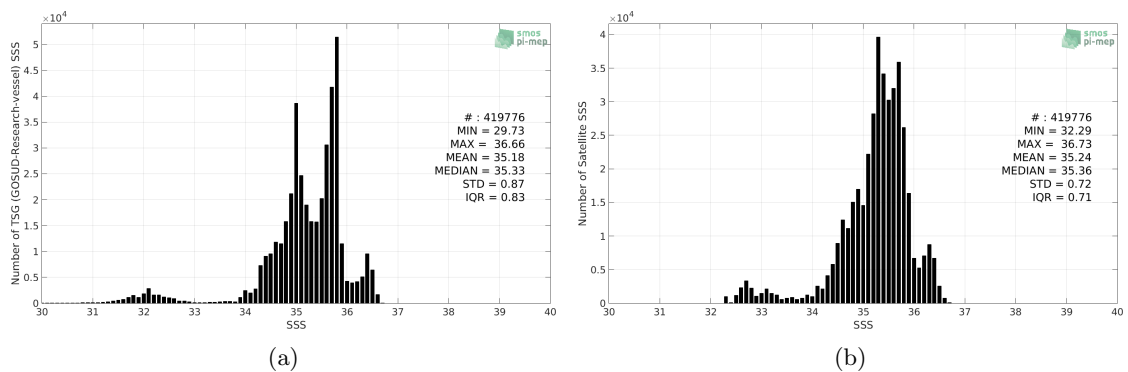
Figure 2: Histograms of SSS from TSG (GOSUD-Research-vessel) (a) and SMOS SSS L3 v4 - 18 Days (CATDS-CECOS-LOCEAN) (b) considering all match-up pairs per bins of 0.1 over the South Pacific Ocean Pi-MEP region and for the full satellite product period.
