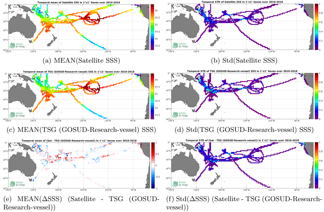
Figure 6: Temporal mean (left) and Std (right) of SSS from SMOS SSS L3 v4 - 18 Days (CATDS-CECOS-LOCEAN) (top), TSG (GOSUD-Research-vessel) (middle), and of \Delta SSS (Satellite - TSG (GOSUD-Research-vessel)). Only match-up pairs are used to generate these maps.
