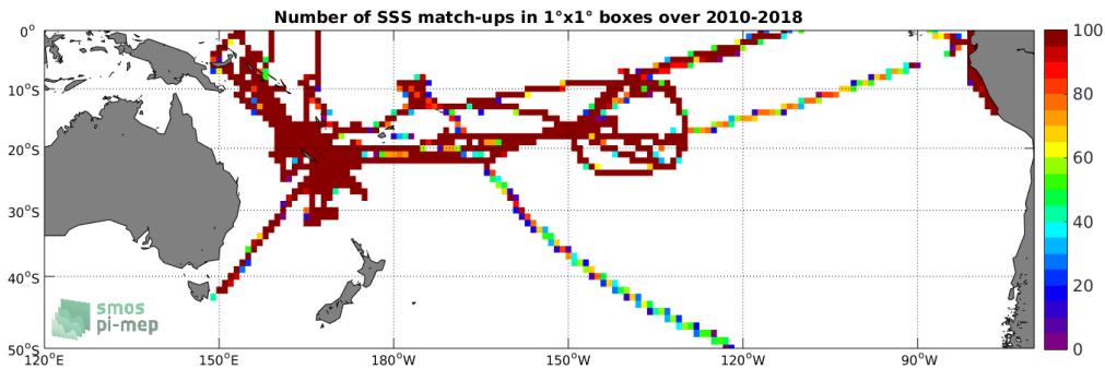
Figure 4: Number of SSS match-ups between TSG (GOSUD-Research-vessel) SSS and the SMOS SSS L3 v4 - 18 Days (CATDS-CECOS-LOCEAN) SSS product for the South Pacific Ocean Pi-MEP region over 1^\circ \times 1^\circ boxes and for the full satellite product period.
