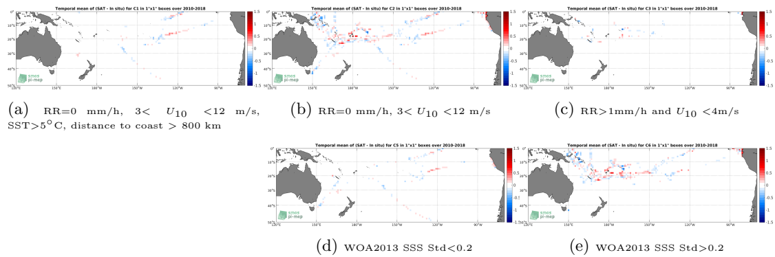
Figure 12: Temporal mean gridded over spatial boxes of size 1^\circ \times 1^\circ of \Delta\text{SSS} (SMOS SSS L3 v4 - 18 Days (CATDS-CECOS-LOCEAN) - TSG (GOSUD-Research-vessel)) for 5 different subdatasets corresponding to:RR=0 mm/h, 3 < U_{10} < 12 m/s, SST>5°C, distance to coast > 800 km (a), RR=0 mm/h, 3 < U_{10} < 12 m/s (b), RR>1mm/h and U_{10} < 4 m/s (c), WOA2013 SSS Std<0.2 (d), WOA2013 SSS Std>0.2 (e).
