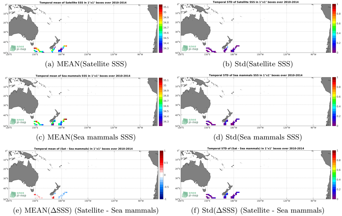
Figure 6: Temporal mean (left) and Std (right) of SSS from SMOS SSS L3 v4 - 18 Days (CATDS-CECOS-LOCEAN) (top), Sea mammals (middle), and of \Delta SSS (Satellite - Sea mammals). Only match-up pairs are used to generate these maps.
