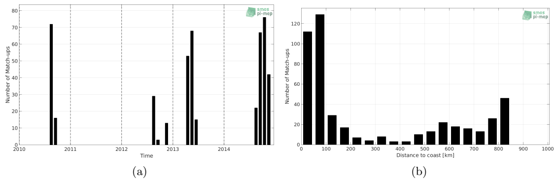
Figure 1: Number of match-ups between Sea mammals and SMOS SSS L3 v4 - 18 Days (CATDS-CECOS-LOCEAN) SSS as a function of time (a) and as function of the distance to coast (b) over the South Pacific Ocean Pi-MEP region and for the full satellite product period.
