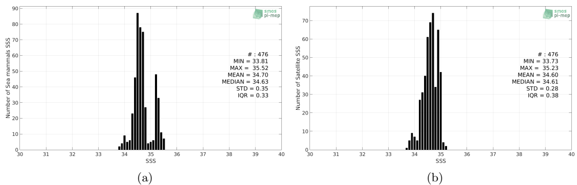
Figure 2: Histograms of SSS from Sea mammals (a) and SMOS SSS L3 v4 - 18 Days (CATDS-CECOS-LOCEAN) (b) considering all match-up pairs per bins of 0.1 over the South Pacific Ocean Pi-MEP region and for the full satellite product period.
