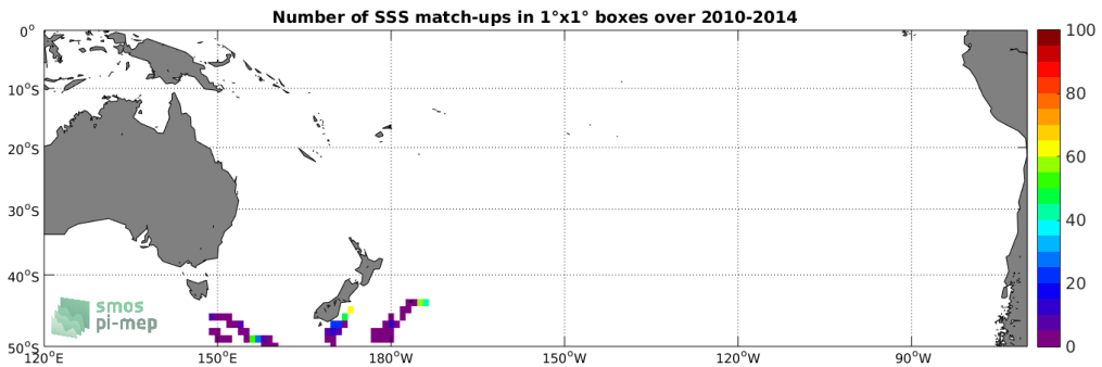
Figure 4: Number of SSS match-ups between Sea mammals SSS and the SMOS SSS L3 v4 - 18 Days (CATDS-CECOS-LOCEAN) SSS product for the South Pacific Ocean Pi-MEP region over 1°x1° boxes and for the full satellite product period.
