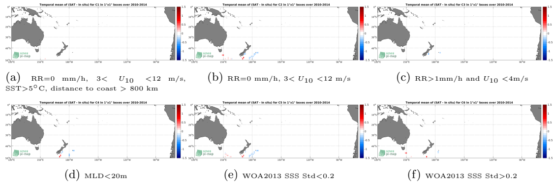
Figure 12: Temporal mean gridded over spatial boxes of size 1^{\circ}\times 1^{\circ} of \Delta\text{SSS} (SMOS SSS L3 v4 - 18 Days (CATDS-CECOS-LOCEAN) - Sea mammals) for 6 different subdatasets corresponding to:RR=0 mm/h, 3 < U_{10} < 12 m/s, SST >5^{\circ}\text{C} , distance to coast > 800 km (a), RR=0 mm/h, 3 < U_{10} < 12 m/s (b), RR >1 mm/h and U_{10} < 4 m/s (c),MLD <20 m (d),WOA2013 SSS Std <0.2 (e),WOA2013 SSS Std >0.2 (f).
