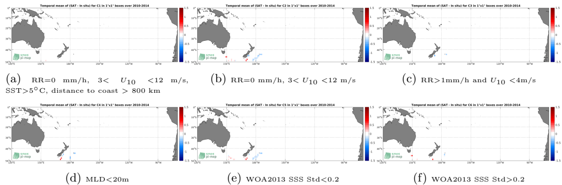
Figure 12: Temporal mean gridded over spatial boxes of size 1^{\circ}\times 1^{\circ} of \Delta\text{SSS} (SMOS-L3-CATDS-CECOS-LOCEAN-V4-18DAYS-25KM - Sea mammals) for 6 different subdatasets corresponding to:RR=0 mm/h, 3 < U_{10} < 12 m/s, SST >5^{\circ}\text{C} , distance to coast > 800 km (a), RR=0 mm/h, 3 < U_{10} < 12 m/s (b), RR >1\text{mm/h} and U_{10} < 4\text{m/s} (c),MLD <20\text{m} (d),WOA2013 SSS Std <0.2 (e),WOA2013 SSS Std >0.2 (f).
