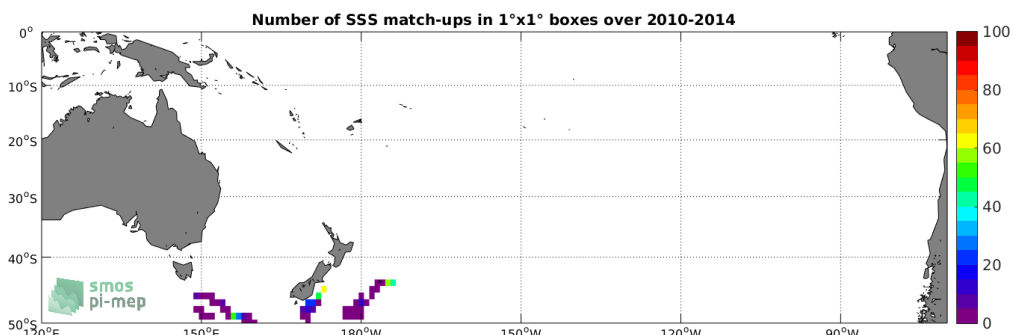
Figure 4: Number of SSS match-ups between Sea mammals SSS and the SMOS-L3-CATDS-CECOS-LOCEAN-V4-18DAYS-25KM SSS product for the South Pacific Ocean Pi-MEP region over 1°x1° boxes and for the full satellite product period.
