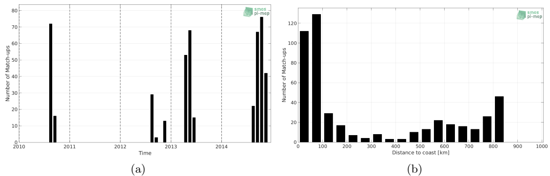
Figure 1: Number of match-ups between Sea mammals and SMOS-L3-CATDS-CECOS-LOCEAN-V4-18DAYS-25KM SSS as a function of time (a) and as function of the distance to coast (b) over the South Pacific Ocean Pi-MEP region and for the full satellite product period.
