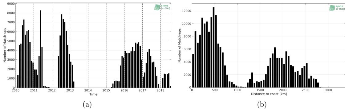
Figure 1: Number of match-ups between Surface drifters and SMOS SSS L3 v4 - 18 Days (CATDS-CECOS-LOCEAN) SSS as a function of time (a) and as function of the distance to coast (b) over the South Pacific Ocean Pi-MEP region and for the full satellite product period.
