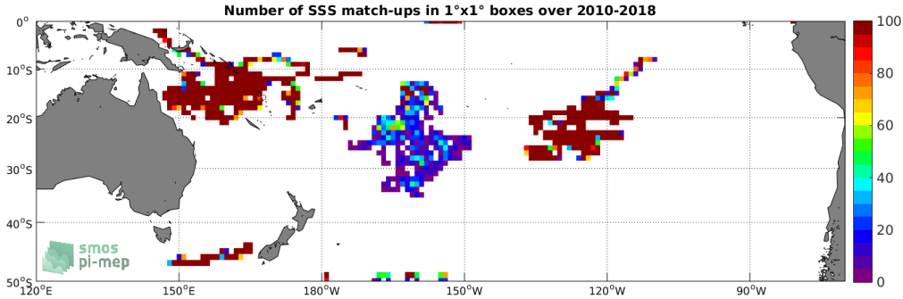
Figure 3: Number of SSS match-ups between Surface drifters SSS and the SMOS SSS L3 v4 - 18 Days (CATDS-CECOS-LOCEAN) SSS product for the South Pacific Ocean Pi-MEP region over 1^\circ \times 1^\circ boxes and for the full satellite product period.
