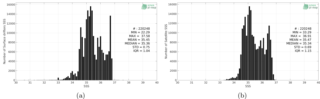
Figure 2: Histograms of SSS from Surface drifters (a) and SMOS SSS L3 v4 - 18 Days (CATDS-CECOS-LOCEAN) (b) considering all match-up pairs per bins of 0.1 over the South Pacific Ocean Pi-MEP region and for the full satellite product period.
