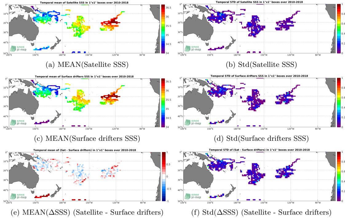
Figure 5: Temporal mean (left) and Std (right) of SSS from SMOS SSS L3 v4 - 18 Days (CATDS-CECOS-LOCEAN) (top), Surface drifters (middle), and of \Delta SSS (Satellite - Surface drifters). Only match-up pairs are used to generate these maps.
