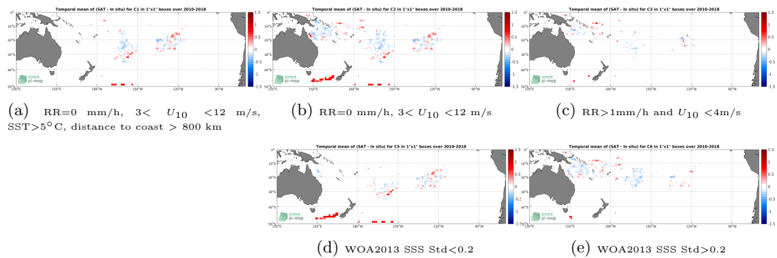
Figure 11: Temporal mean gridded over spatial boxes of size 1^\circ \times 1^\circ of \Delta\text{SSS} (SMOS SSS L3 v4 - 18 Days (CATDS-CECOS-LOCEAN) - Surface drifters) for 5 different subdatasets corresponding to:RR=0 mm/h, 3 < U_{10} < 12 m/s, SST >5^\circ\text{C} , distance to coast > 800 km (a), RR=0 mm/h, 3 < U_{10} < 12 m/s (b), RR >1 mm/h and U_{10} < 4 m/s (c), WOA2013 SSS Std <0.2 (d), WOA2013 SSS Std >0.2 (e).
