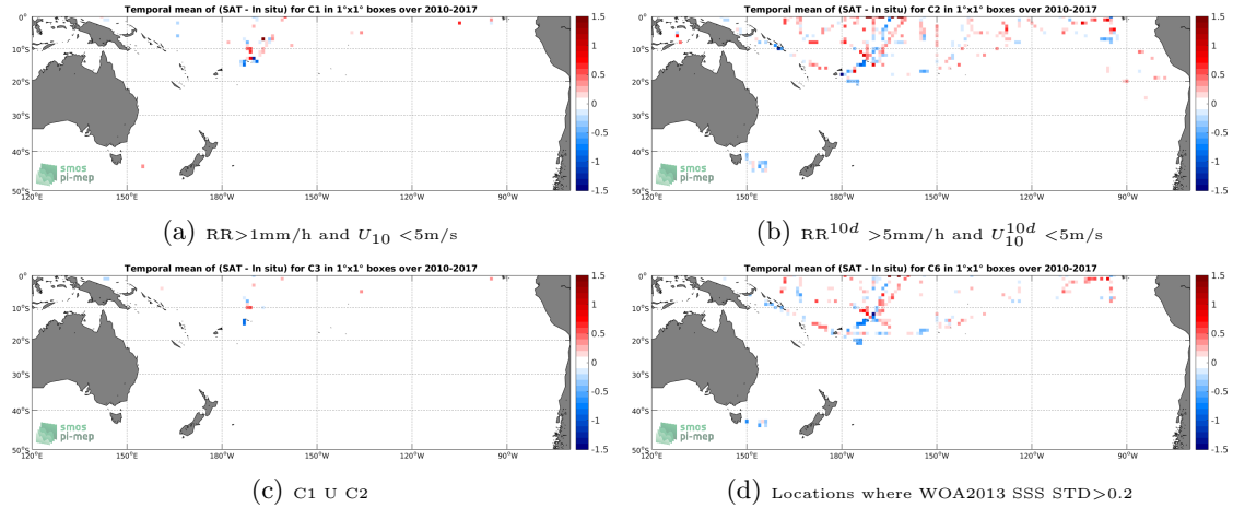
Figure 12: Temporal mean gridded over spatial boxes of size 1^\circ \times 1^\circ of \Delta SSS (SMOS-L3-CATDS-CECOS-LOCEAN-V3-9DAYS-25KM - TSG-SAMOS) for 4 different subdatasets corresponding to: RR > 1\text{mm/h} and U_{10} < 5\text{m/s} (a), RR^{10d} > 5\text{mm/h} and U_{10}^{10d} < 5\text{m/s} (b), C1 U C2 (c), Locations where WOA2013 SSS STD > 0.2 (d).
