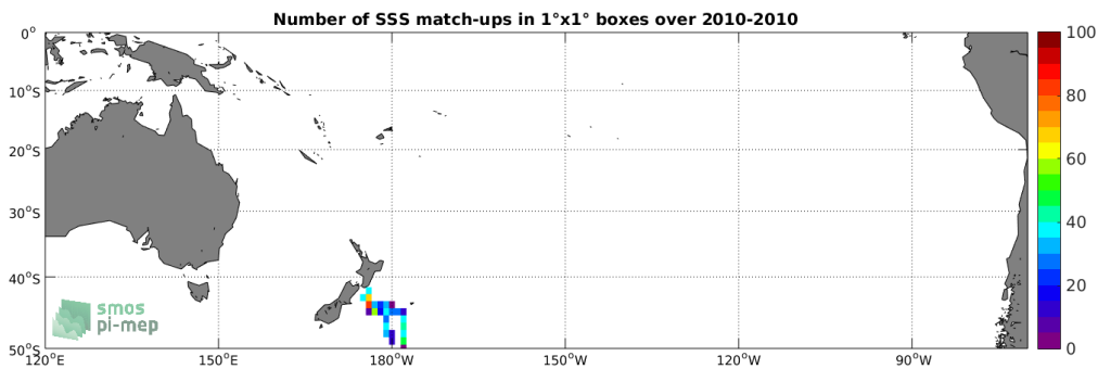
Figure 4: Number of SSS match-ups between TSG-POLARSTERN SSS and the SMOS-L3-CATDS-CECOS-LOCEAN-V3-9DAYS-25KM SSS product for the South Pacific Ocean Pi-MEP region over 1^\circ \times 1^\circ boxes and for the full satellite product period.
