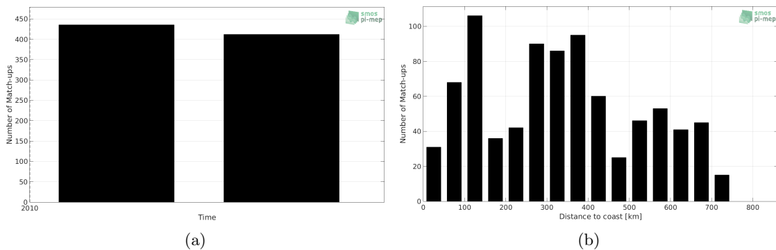
Figure 1: Number of match-ups between TSG-POLARSTERN and SMOS-L3-CATDS-CECOS-LOCEAN-V3-9DAYS-25KM SSS as a function of time (a) and as function of the distance to coast (b) over the South Pacific Ocean Pi-MEP region and for the full satellite product period.
