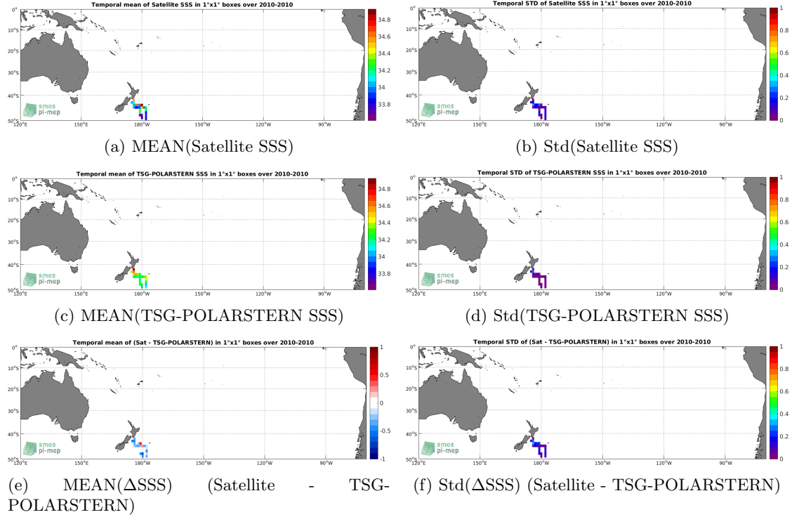
Figure 6: Temporal mean (left) and Std (right) of SSS from SMOS-L3-CATDS-CECOS-LOCEAN-V3-9DAYS-25KM (top), TSG-POLARSTERN (middle), and of \Delta SSS (Satellite - TSG-POLARSTERN). Only match-up pairs are used to generate these maps.
