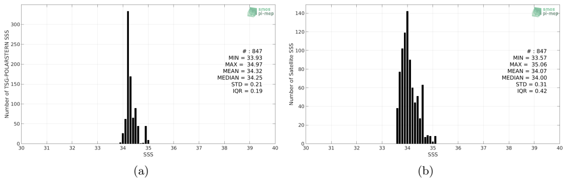
Figure 2: Histograms of SSS from TSG-POLARSTERN (a) and SMOS-L3-CATDS-CECOS-LOCEAN-V3-9DAYS-25KM (b) considering all match-up pairs per bins of 0.1 over the South Pacific Ocean Pi-MEP region and for the full satellite product period.
