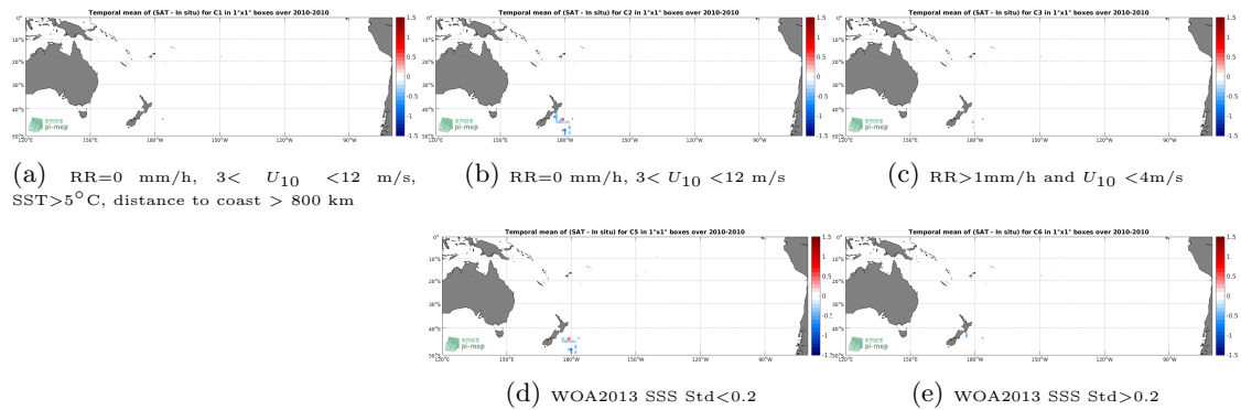
Figure 12: Temporal mean gridded over spatial boxes of size 1^\circ \times 1^\circ of \Delta SSS (SMOS-L3-CATDS-CECOS-LOCEAN-V3-9DAYS-25KM - TSG-POLARSTERN) for 5 different subdatasets corresponding to:RR=0 mm/h, 3 < U_{10} < 12 m/s, SST >5^\circ C, distance to coast > 800 km (a), RR=0 mm/h, 3 < U_{10} < 12 m/s (b), RR >1 mm/h and U_{10} < 4 m/s (c), WOA2013 SSS Std <0.2 (d), WOA2013 SSS Std >0.2 (e).
