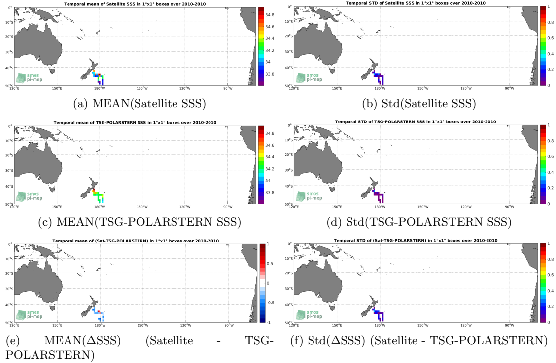
Figure 6: Temporal mean (left) and Std (right) of SSS from SMOS-L3-CATDS-CECOS-LOCEAN-V3-9DAYS-25KM (top), TSG-POLARSTERN (middle), and of \Delta SSS (Satellite - TSG-POLARSTERN). Only match-up pairs are used to generate these maps.
