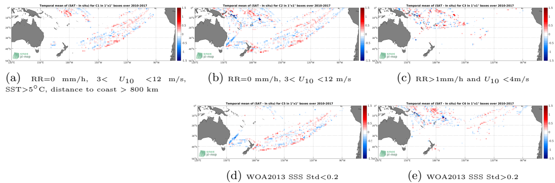
Figure 12: Temporal mean gridded over spatial boxes of size 1^\circ \times 1^\circ of \Delta SSS (SMOS-L3-CATDS-CECOS-LOCEAN-V3-9DAYS-25KM - TSG-LEGOS-DM) for 5 different subdatasets corresponding to:RR=0 mm/h, 3 < U_{10} < 12 m/s, SST >5^\circ\text{C} , distance to coast > 800 km (a), RR=0 mm/h, 3 < U_{10} < 12 m/s (b), RR >1 mm/h and U_{10} < 4 m/s (c), WOA2013 SSS Std <0.2 (d), WOA2013 SSS Std >0.2 (e).
