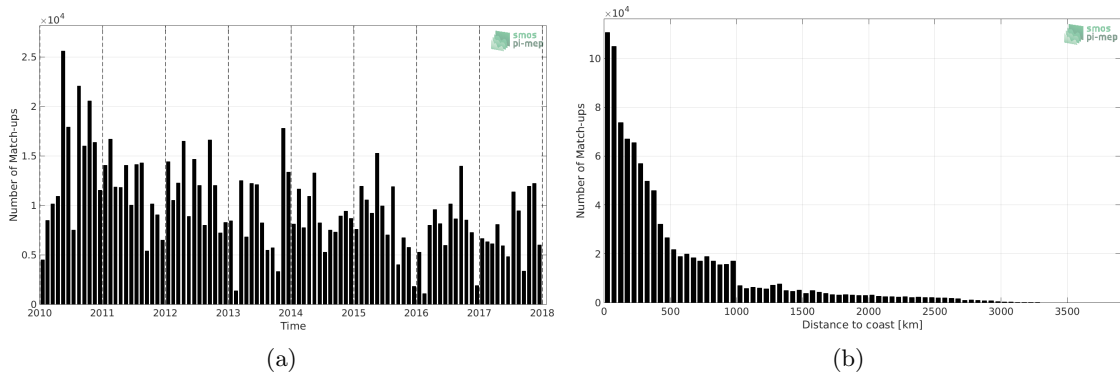
Figure 1: Number of match-ups between TSG-LEGOS-DM and SMOS-L3-CATDS-CECOS-LOCEAN-V3-9DAYS-25KM SSS as a function of time (a) and as function of the distance to coast (b) over the South Pacific Ocean Pi-MEP region and for the full satellite product period.
