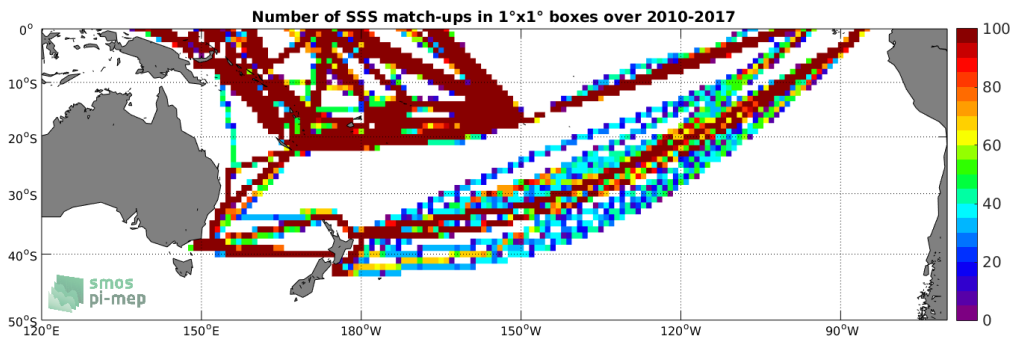
Figure 4: Number of SSS match-ups between TSG-LEGOS-DM SSS and the SMOS-L3-CATDS-CECOS-LOCEAN-V3-9DAYS-25KM SSS product for the South Pacific Ocean Pi-MEP region over 1^\circ \times 1^\circ boxes and for the full satellite product period.
