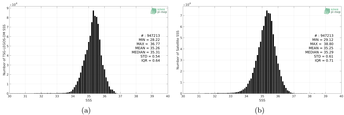
Figure 2: Histograms of SSS from TSG-LEGOS-DM (a) and SMOS-L3-CATDS-CECOS-LOCEAN-V3-9DAYS-25KM (b) considering all match-up pairs per bins of 0.1 over the South Pacific Ocean Pi-MEP region and for the full satellite product period.
