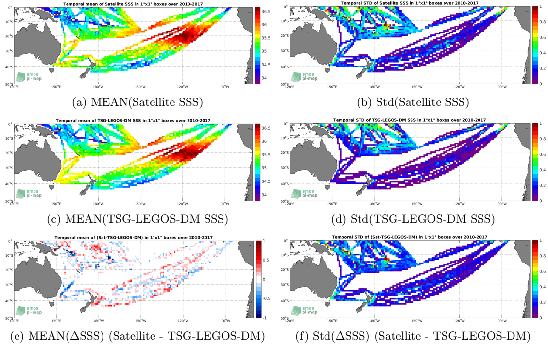
Figure 6: Temporal mean (left) and Std (right) of SSS from SMOS-L3-CATDS-CECOS-LOCEAN-V3-9DAYS-25KM (top), TSG-LEGOS-DM (middle), and of \Delta SSS (Satellite - TSG-LEGOS-DM). Only match-up pairs are used to generate these maps.
