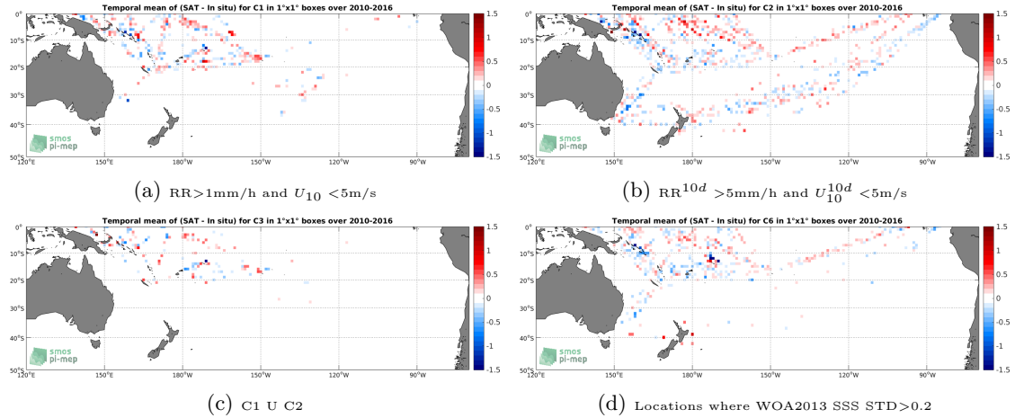
Figure 12: Temporal mean gridded over spatial boxes of size 1^\circ \times 1^\circ of \Delta SSS (SMOS-L3-CATDS-CECOS-LOCEAN-V3-9DAYS-25KM - TSG-LEGOS-DM) for 4 different subdatasets corresponding to: RR > 1mm/h and U_{10} < 5\text{m/s} (a), RR^{10d} > 5\text{mm/h} and U_{10}^{10d} < 5\text{m/s} (b), C1 U C2 (c), Locations where WOA2013 SSS STD > 0.2 (d).
