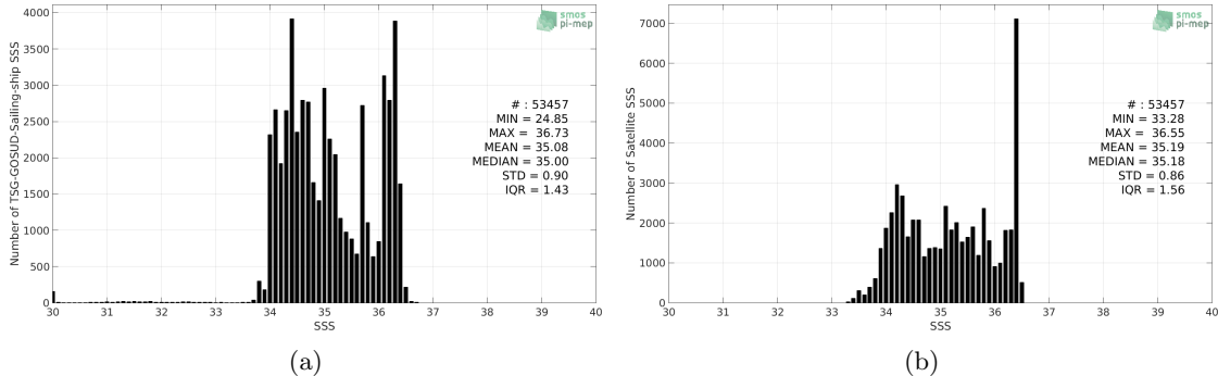
Figure 2: Histograms of SSS from TSG-GOSUD-Sailing-ship (a) and SMOS-L3-CATDS-CECOS-LOCEAN-V3-9DAYS-25KM (b) considering all match-up pairs per bins of 0.1 over the South Pacific Ocean Pi-MEP region and for the full satellite product period.
