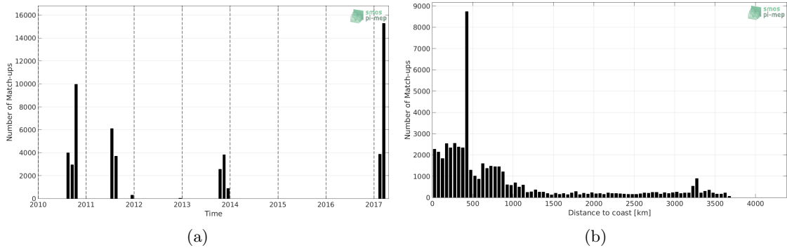
Figure 1: Number of match-ups between TSG-GOSUD-Sailing-ship and SMOS-L3-CATDS-CECOS-LOCEAN-V3-9DAYS-25KM SSS as a function of time (a) and as function of the distance to coast (b) over the South Pacific Ocean Pi-MEP region and for the full satellite product period.
