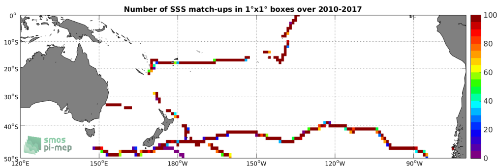
Figure 4: Number of SSS match-ups between TSG-GOSUD-Sailing-ship SSS and the SMOS-L3-CATDS-CECOS-LOCEAN-V3-9DAYS-25KM SSS product for the South Pacific Ocean Pi-MEP region over 1^\circ \times 1^\circ boxes and for the full satellite product period.
