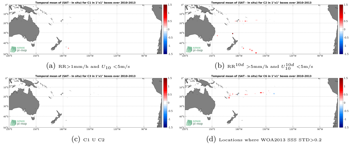
Figure 12: Temporal mean gridded over spatial boxes of size 1^\circ \times 1^\circ of \Delta SSS (SMOS-L3-CATDS-CECOS-LOCEAN-V3-9DAYS-25KM - TSG-GOSUD-Sailing-ship) for 4 different subdatasets corresponding to: RR > 1mm/h and U_{10} < 5\text{m/s} (a), RR^{10d} > 5\text{mm/h} and U_{10}^{10d} < 5\text{m/s} (b), C1 U C2 (c), Locations where WOA2013 SSS STD > 0.2 (d).
