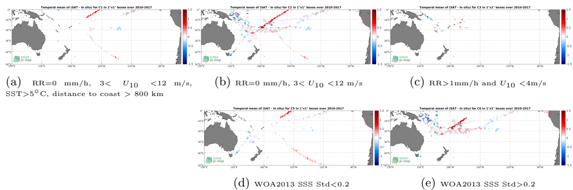
Figure 12: Temporal mean gridded over spatial boxes of size 1^\circ \times 1^\circ of \Delta SSS (SMOS-L3-CATDS-CECOS-LOCEAN-V3-9DAYS-25KM - TSG-GOSUD-Research-vessel) for 5 different subdatasets corresponding to:RR=0 mm/h, 3 < U_{10} < 12 m/s, SST>5°C, distance to coast > 800 km (a), RR=0 mm/h, 3 < U_{10} < 12 m/s (b), RR>1mm/h and U_{10} < 4 m/s (c), WOA2013 SSS Std<0.2 (d), WOA2013 SSS Std>0.2 (e).
