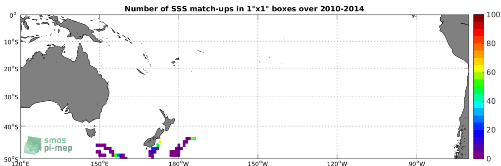
Figure 4: Number of SSS match-ups between Sea mammals SSS and the SMOS-L3-CATDS-CECOS-LOCEAN-V3-9DAYS-25KM SSS product for the South Pacific Ocean Pi-MEP region over 1^\circ \times 1^\circ boxes and for the full satellite product period.
