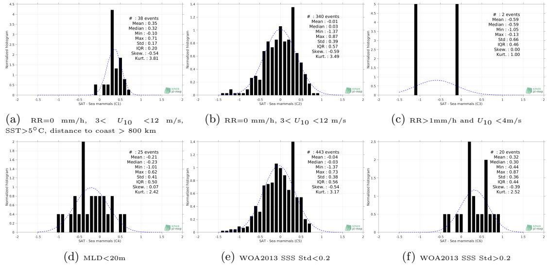
Figure 13: Normalized histogram of \Delta SSS (SMOS-L3-CATDS-CECOS-LOCEAN-V3-9DAYS-25KM - Sea mammals) for 6 different subdatasets corresponding to: RR=0 mm/h, 3 < U_{10} < 12 m/s, SST>5°C, distance to coast > 800 km (a), RR=0 mm/h, 3 < U_{10} < 12 m/s (b), RR>1mm/h and U_{10} < 4 m/s (c), MLD<20m (d), WOA2013 SSS Std<0.2 (e), WOA2013 SSS Std>0.2 (f).
