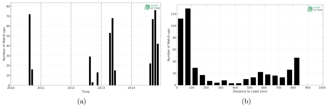
Figure 1: Number of match-ups between Sea mammals and SMOS-L3-CATDS-CECOS-LOCEAN-V3-9DAYS-25KM SSS as a function of time (a) and as function of the distance to coast (b) over the South Pacific Ocean Pi-MEP region and for the full satellite product period.
