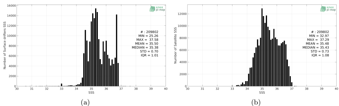
Figure 2: Histograms of SSS from Surface drifters (a) and SMOS-L3-CATDS-CECOS-LOCEAN-V3-9DAYS-25KM (b) considering all match-up pairs per bins of 0.1 over the South Pacific Ocean Pi-MEP region and for the full satellite product period.
