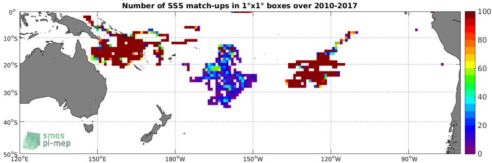
Figure 3: Number of SSS match-ups between Surface drifters SSS and the SMOS-L3-CATDS-CECOS-LOCEAN-V3-9DAYS-25KM SSS product for the South Pacific Ocean Pi-MEP region over 1^\circ \times 1^\circ boxes and for the full satellite product period.
