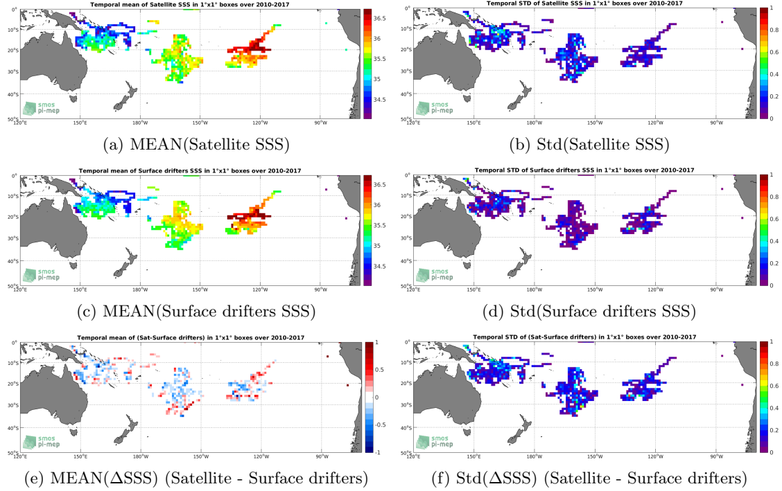
Figure 5: Temporal mean (left) and Std (right) of SSS from SMOS-L3-CATDS-CECOS-LOCEAN-V3-9DAYS-25KM (top), Surface drifters (middle), and of \Delta SSS (Satellite - Surface drifters). Only match-up pairs are used to generate these maps.
