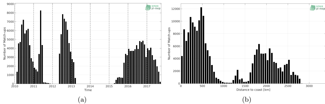
Figure 1: Number of match-ups between Surface drifters and SMOS-L3-CATDS-CECOS-LOCEAN-V3-9DAYS-25KM SSS as a function of time (a) and as function of the distance to coast (b) over the South Pacific Ocean Pi-MEP region and for the full satellite product period.
