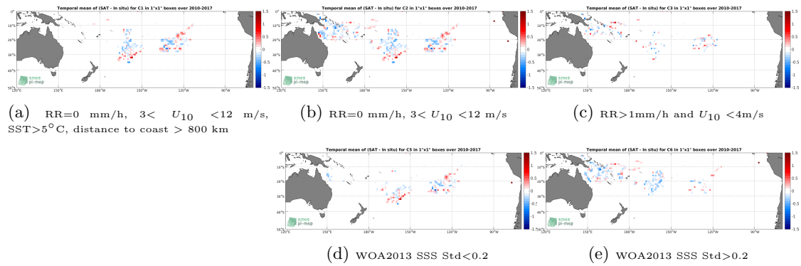
Figure 11: Temporal mean gridded over spatial boxes of size 1^\circ \times 1^\circ of \Delta SSS (SMOS-L3-CATDS-CECOS-LOCEAN-V3-9DAYS-25KM - Surface drifters) for 5 different subdatasets corresponding to:RR=0 mm/h, 3 < U_{10} < 12 m/s, SST >5^\circ C, distance to coast > 800 km (a), RR=0 mm/h, 3 < U_{10} < 12 m/s (b), RR >1 mm/h and U_{10} < 4 m/s (c), WOA2013 SSS Std <0.2 (d), WOA2013 SSS Std >0.2 (e).
