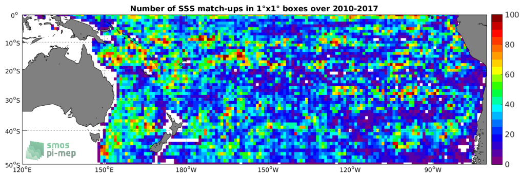
Figure 4: Number of SSS match-ups between Argos SSS and the SMOS-L3-CATDS-CECOS-LOCEAN-V3-9DAYS-25KM SSS product for the South Pacific Ocean Pi-MEP region over 1^\circ \times 1^\circ boxes and for the full satellite product period.
