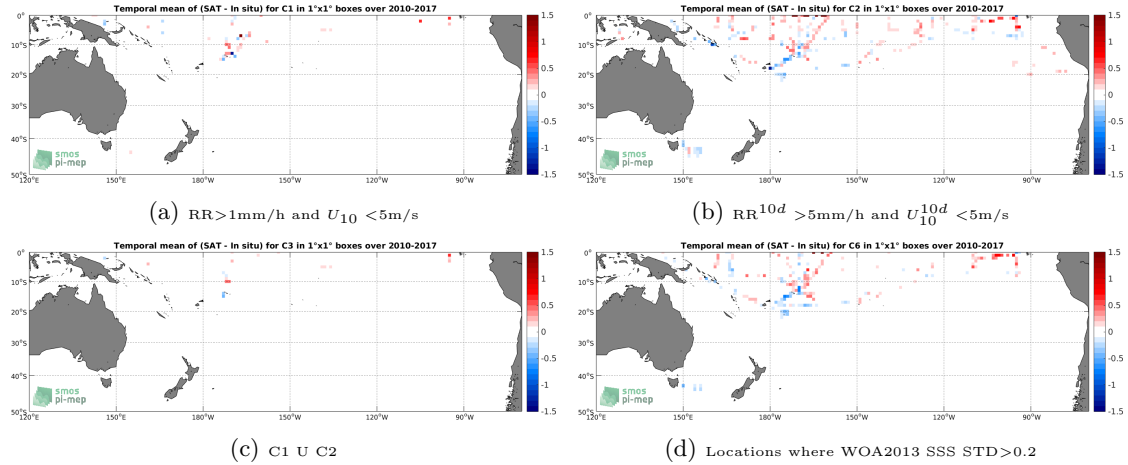
Figure 12: Temporal mean gridded over spatial boxes of size 1^\circ \times 1^\circ of \Delta SSS (SMOS-L3-CATDS-CECOS-LOCEAN-V3-18DAYS-25KM - TSG-SAMOS) for 4 different subdatasets corresponding to: RR > 1\text{mm/h} and U_{10} < 5\text{m/s} (a), RR^{10d} > 5\text{mm/h} and U_{10}^{10d} < 5\text{m/s} (b), C1 U C2 (c), Locations where WOA2013 SSS STD > 0.2 (d).
