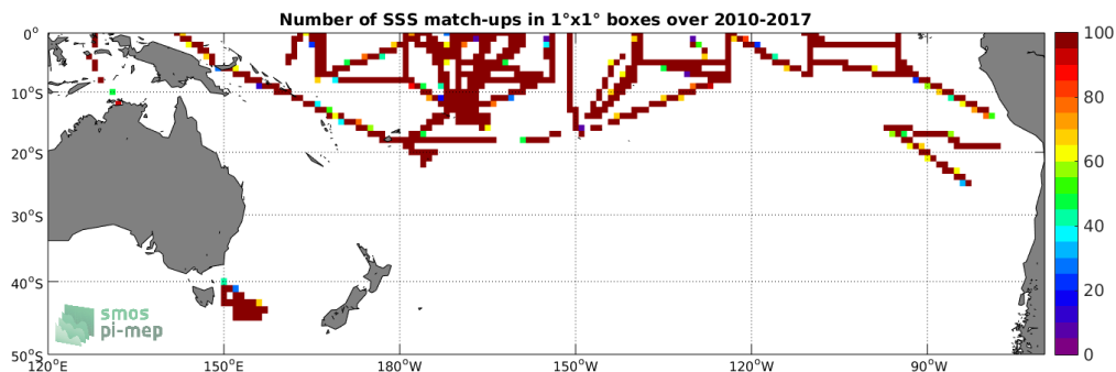
Figure 4: Number of SSS match-ups between TSG-SAMOS SSS and the SMOS-L3-CATDS-CECOS-LOCEAN-V3-18DAYS-25KM SSS product for the South Pacific Ocean Pi-MEP region over 1^\circ \times 1^\circ boxes and for the full satellite product period.
