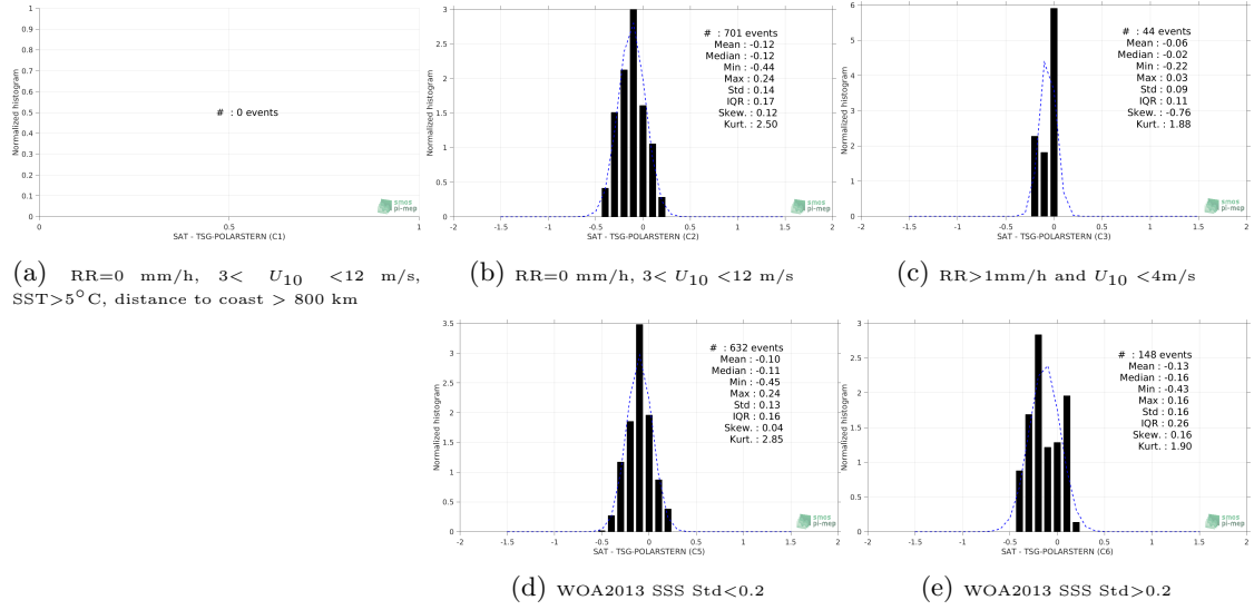
Figure 13: Normalized histogram of \Delta\text{SSS} (SMOS-L3-CATDS-CECOS-LOCEAN-V3-18DAYS-25KM - TSG-POLARSTERN) for 5 different subdatasets corresponding to: RR=0 mm/h, 3 < U_{10} < 12 m/s, SST > 5^{\circ}\text{C} , distance to coast > 800 km (a), RR=0 mm/h, 3 < U_{10} < 12 m/s (b), RR > 1\text{mm/h} and U_{10} < 4\text{m/s} (c), WOA2013 SSS Std <0.2 (d), WOA2013 SSS Std >0.2 (e).
