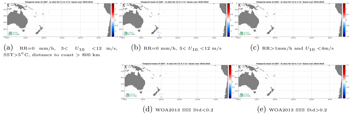
Figure 12: Temporal mean gridded over spatial boxes of size 1^\circ \times 1^\circ of \Delta SSS (SMOS-L3-CATDS-CECOS-LOCEAN-V3-18DAYS-25KM - TSG-POLARSTERN) for 5 different subdatasets corresponding to: RR=0 mm/h, 3 < U_{10} < 12 m/s, SST > 5^\circ\text{C} , distance to coast > 800 km (a), RR=0 mm/h, 3 < U_{10} < 12 m/s (b), RR > 1 mm/h and U_{10} < 4 m/s (c), WOA2013 SSS Std < 0.2 (d), WOA2013 SSS Std > 0.2 (e).
