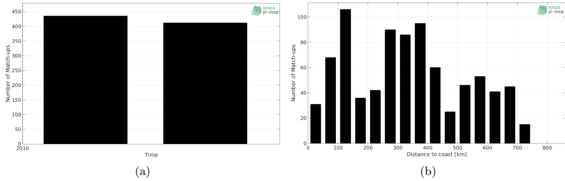
Figure 1: Number of match-ups between TSG-POLARSTERN and SMOS-L3-CATDS-CECOS-LOCEAN-V3-18DAYS-25KM SSS as a function of time (a) and as function of the distance to coast (b) over the South Pacific Ocean Pi-MEP region and for the full satellite product period.
