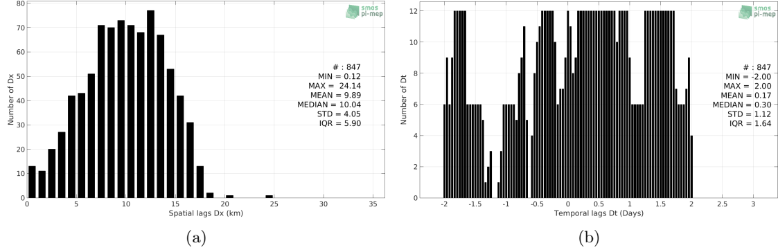
Figure 5: Histograms of the spatial (a) and temporal (b) lags between the time of the TSG-POLARSTERN measurements and the date of the corresponding SMOS-L3-CATDS-CECOS-LOCEAN-V3-18DAYS-25KM SSS product.
