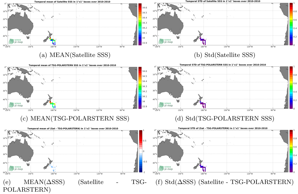
Figure 6: Temporal mean (left) and Std (right) of SSS from SMOS-L3-CATDS-CECOS-LOCEAN-V3-18DAYS-25KM (top), TSG-POLARSTERN (middle), and of \Delta SSS (Satellite - TSG-POLARSTERN). Only match-up pairs are used to generate these maps.
