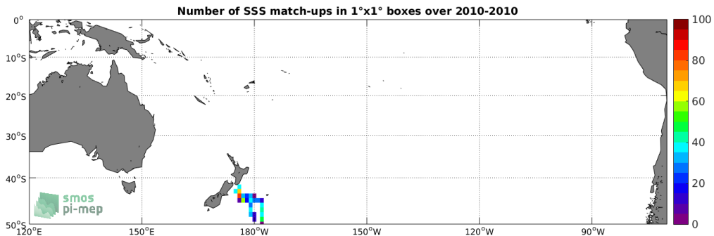
Figure 4: Number of SSS match-ups between TSG-POLARSTERN SSS and the SMOS-L3-CATDS-CECOS-LOCEAN-V3-18DAYS-25KM SSS product for the South Pacific Ocean Pi-MEP region over 1°x1° boxes and for the full satellite product period.
