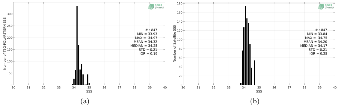
Figure 2: Histograms of SSS from TSG-POLARSTERN (a) and SMOS-L3-CATDS-CECOS-LOCEAN-V3-18DAYS-25KM (b) considering all match-up pairs per bins of 0.1 over the South Pacific Ocean Pi-MEP region and for the full satellite product period.
