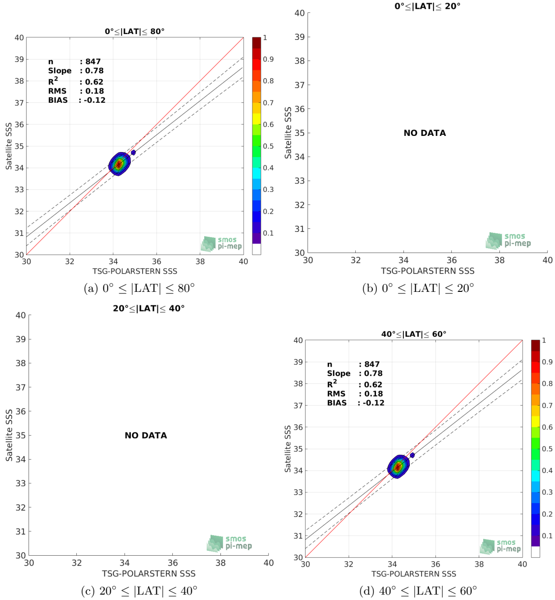
Figure 9: Contour maps of the concentration of SMOS-L3-CATDS-CECOS-LOCEAN-V3-18DAYS-25KM SSS (y-axis) versus TSG-POLARSTERN SSS (x-axis) at match-up pairs for different latitude bands. For each plot, the red line shows x=y . The black thin and dashed lines indicate a linear fit through the data cloud and the \pm 95\% confidence levels, respectively. The number match-up pairs n , the slope and R^2 coefficient of the linear fit, the root mean square (RMS) and the mean bias between satellite and in situ data are indicated for each latitude band in each plots.
