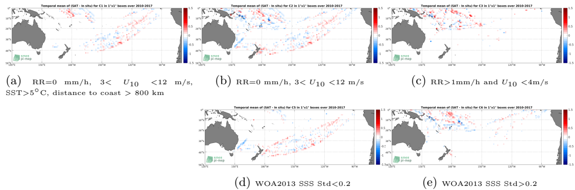
Figure 12: Temporal mean gridded over spatial boxes of size 1^\circ \times 1^\circ of \Delta SSS (SMOS-L3-CATDS-CECOS-LOCEAN-V3-18DAYS-25KM - TSG-LEGOS-DM) for 5 different subdatasets corresponding to:RR=0 mm/h, 3 < U_{10} < 12 m/s, SST >5^\circ C, distance to coast > 800 km (a), RR=0 mm/h, 3 < U_{10} < 12 m/s (b), RR >1 mm/h and U_{10} < 4 m/s (c), WOA2013 SSS Std <0.2 (d), WOA2013 SSS Std >0.2 (e).
