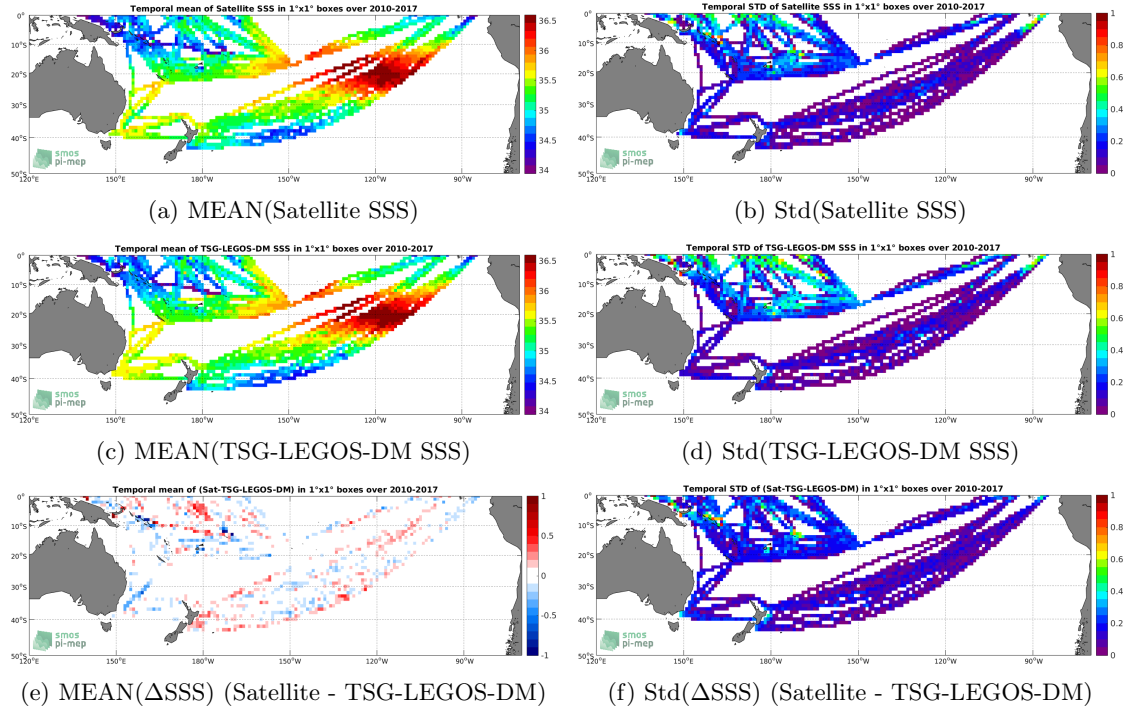
Figure 6: Temporal mean (left) and Std (right) of SSS from SMOS-L3-CATDS-CECOS-LOCEAN-V3-18DAYS-25KM satellite SSS product (in black) and the TSG-LEGOS-DM in situ dataset (in blue) at the collected Pi-MEP match-up pairs. Only match-up pairs are used to generate these maps.
